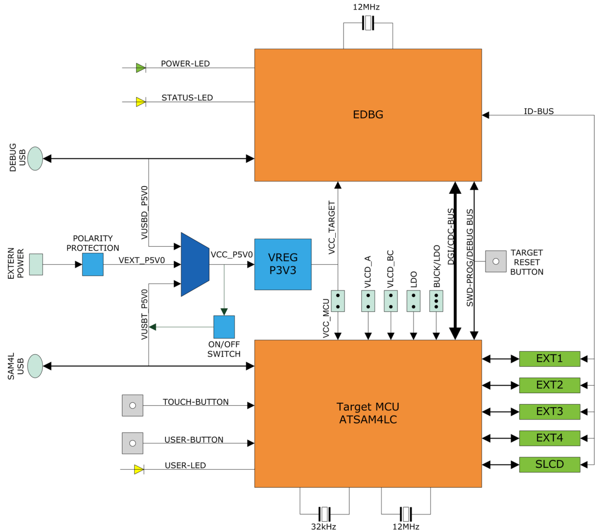
Figure 1-2 SAM4L Xplained Pro Block Diagram
