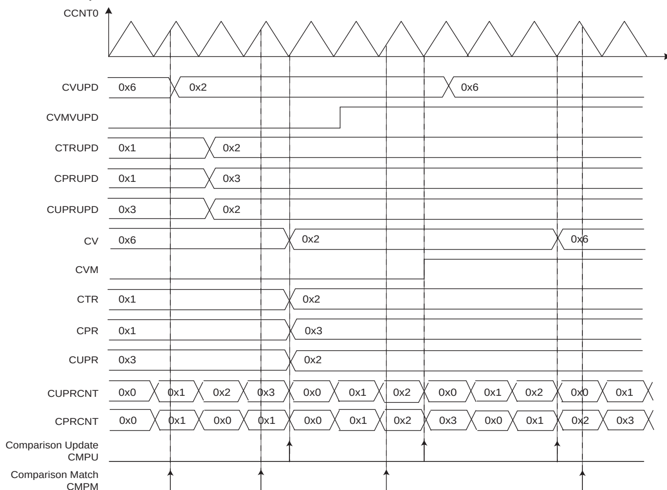
Figure 39-18. Comparison Waveform
