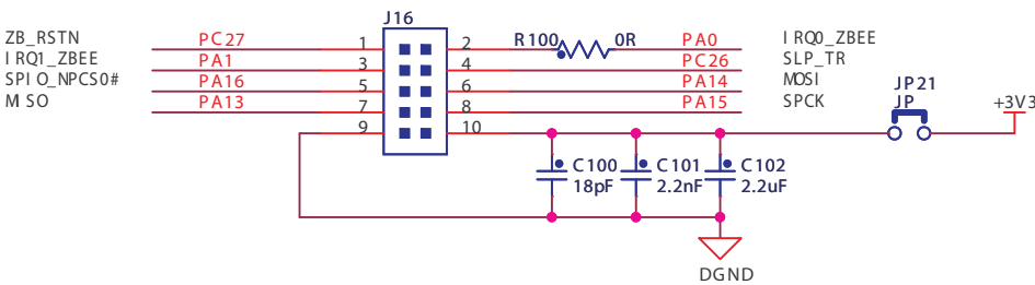
Figure 4-22. ZigBee
