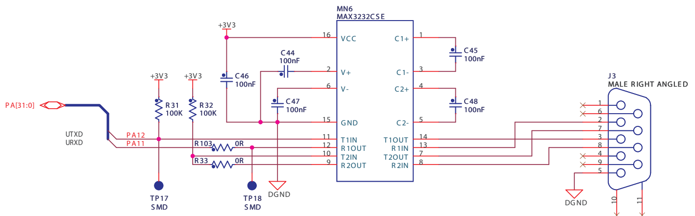
Figure 4-8. UART
