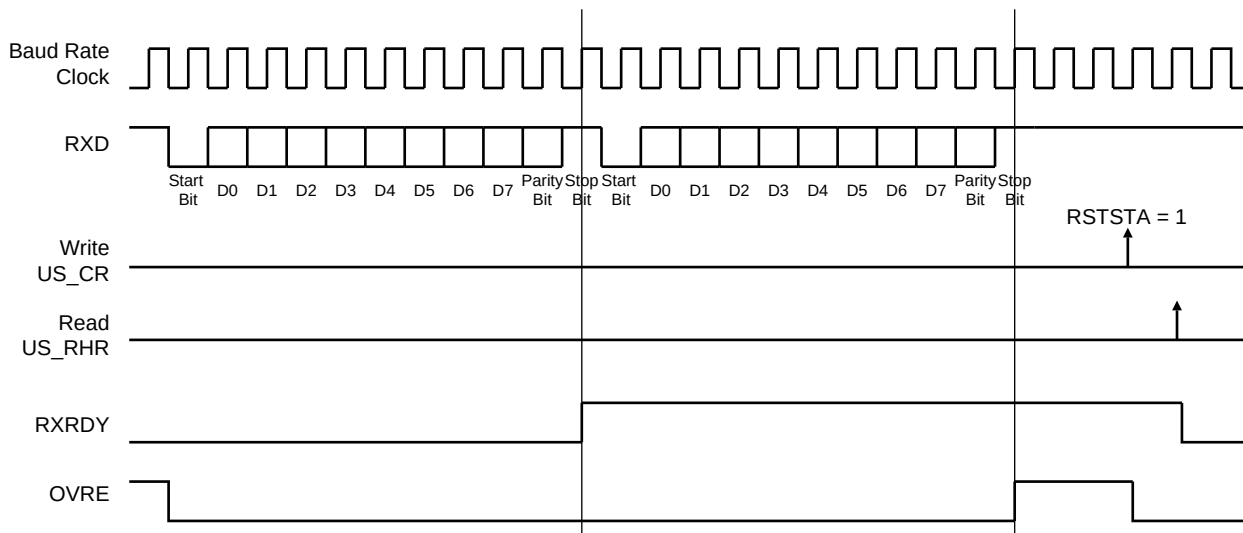
Figure 31-11. Receiver Status
