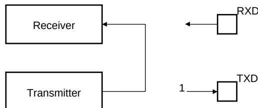
Figure 31-32. Local Loopback Mode Configuration
