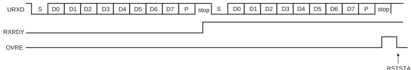
Figure 30-6. Receiver Overrun
