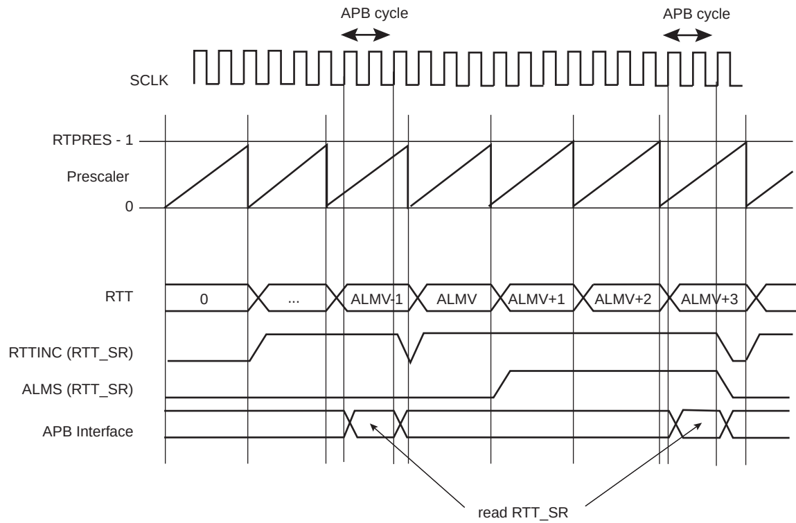
Figure 14-2. RTT Counting
