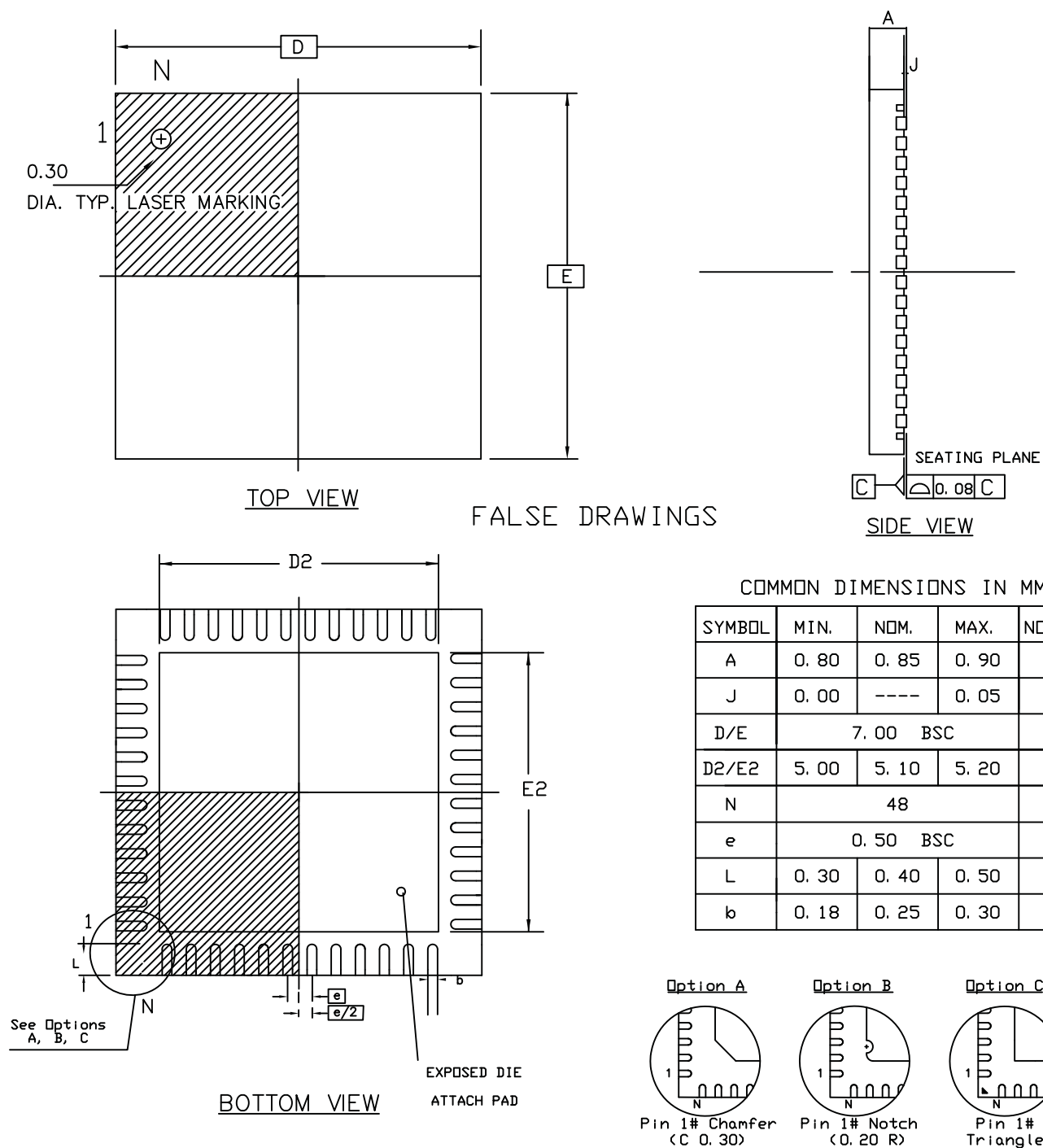
Figure 37-4. 48-pad QFN Package
