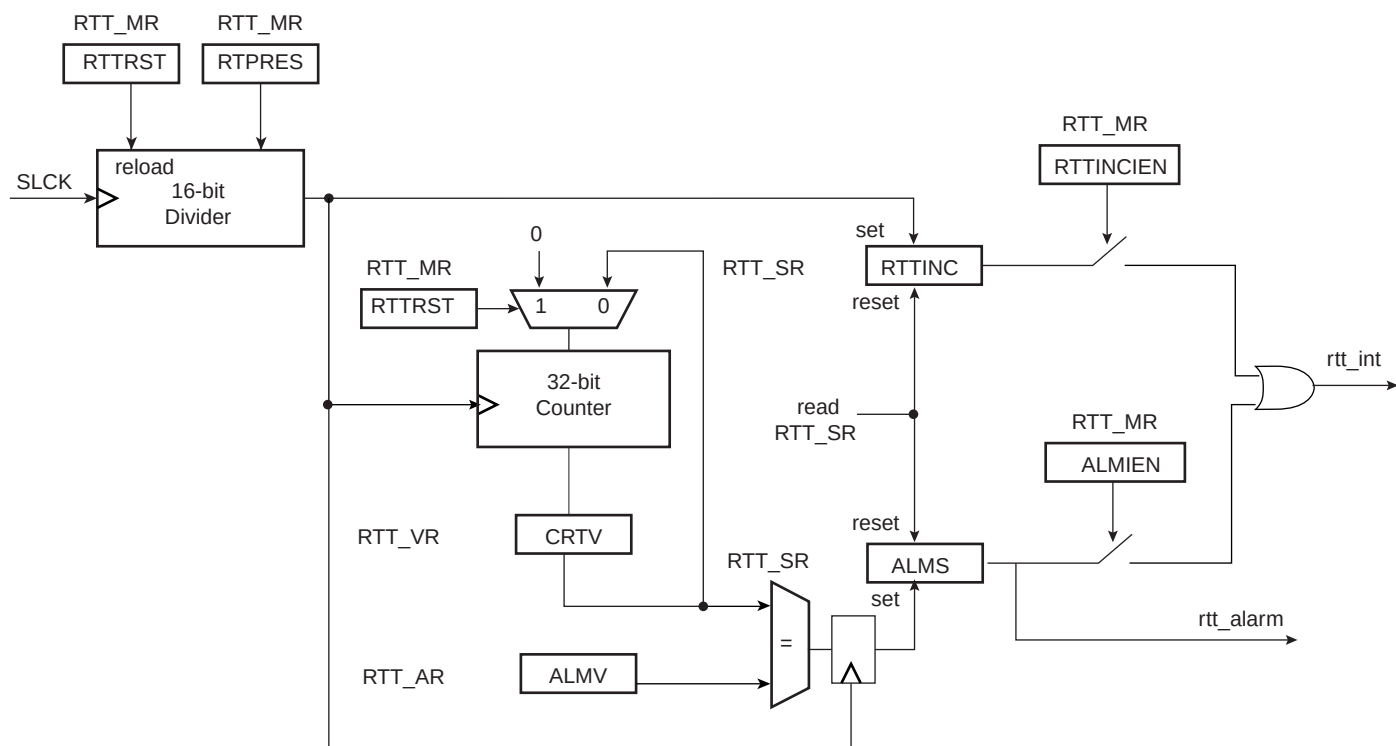
Figure 14-1. Real-time Timer
