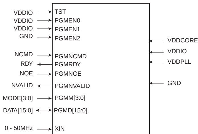
Figure 20-2. SAM3NB/C (64/100 pins) Parallel Programming Interface
