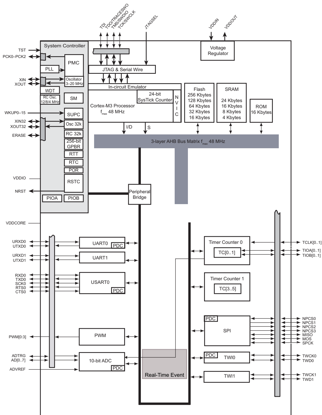
Figure 2-3. SAM3N 48-pin version Block Diagram
