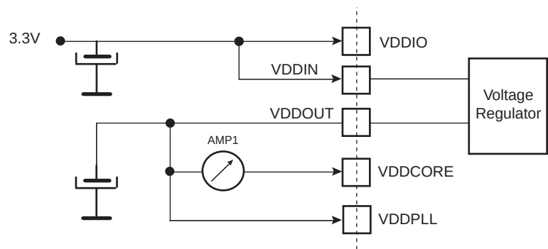
Figure 36-8. Active Mode Measurement Setup
