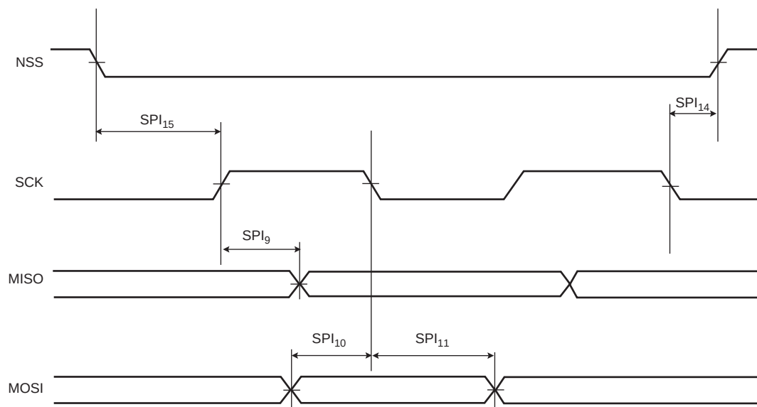
Figure 36-22. USART SPI Slave mode: (Mode 0 or 3)
