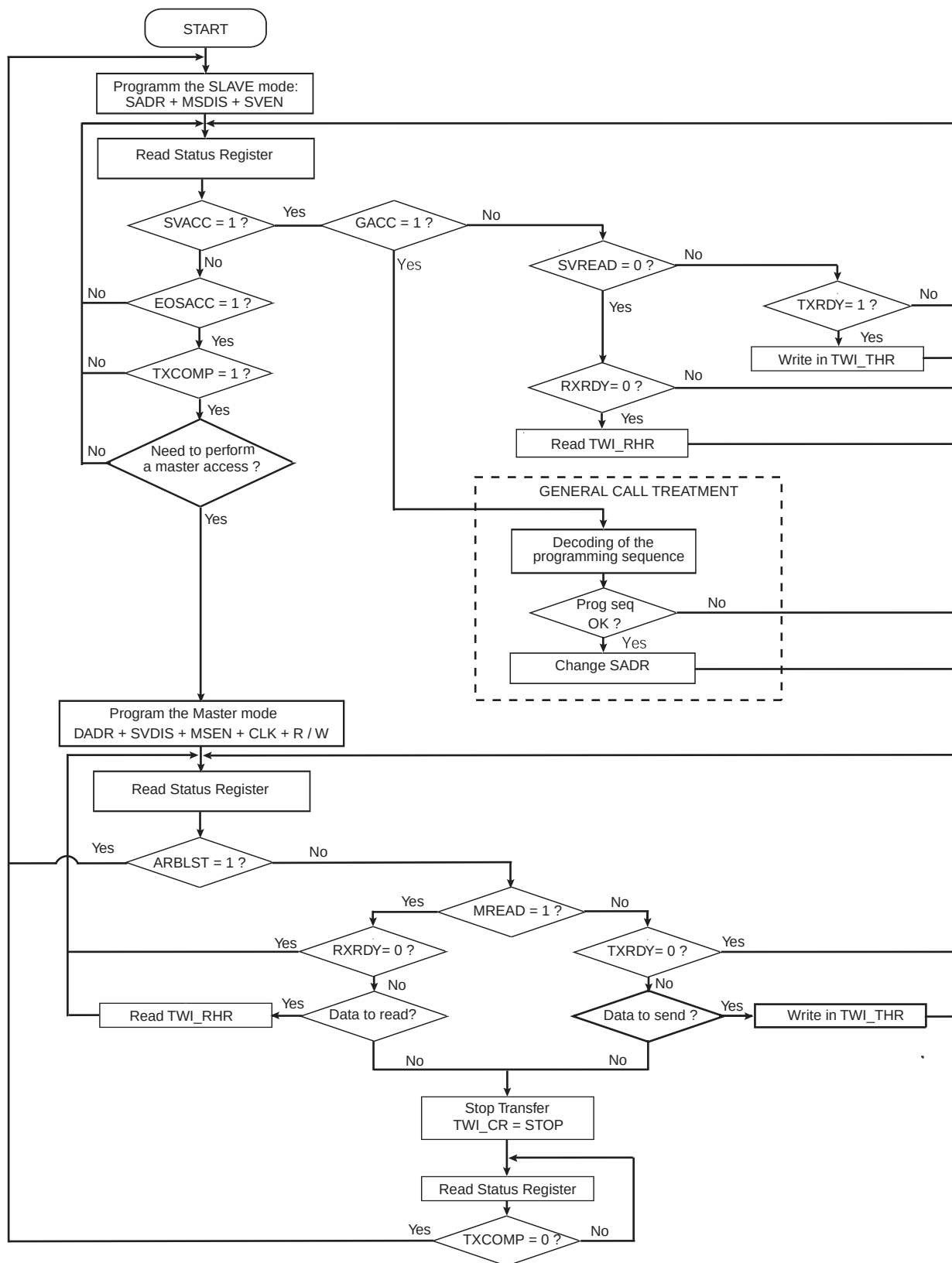
Figure 29-23. Multi-master Flowchart
