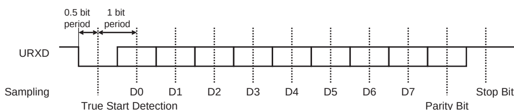
Figure 30-4. Character Reception
