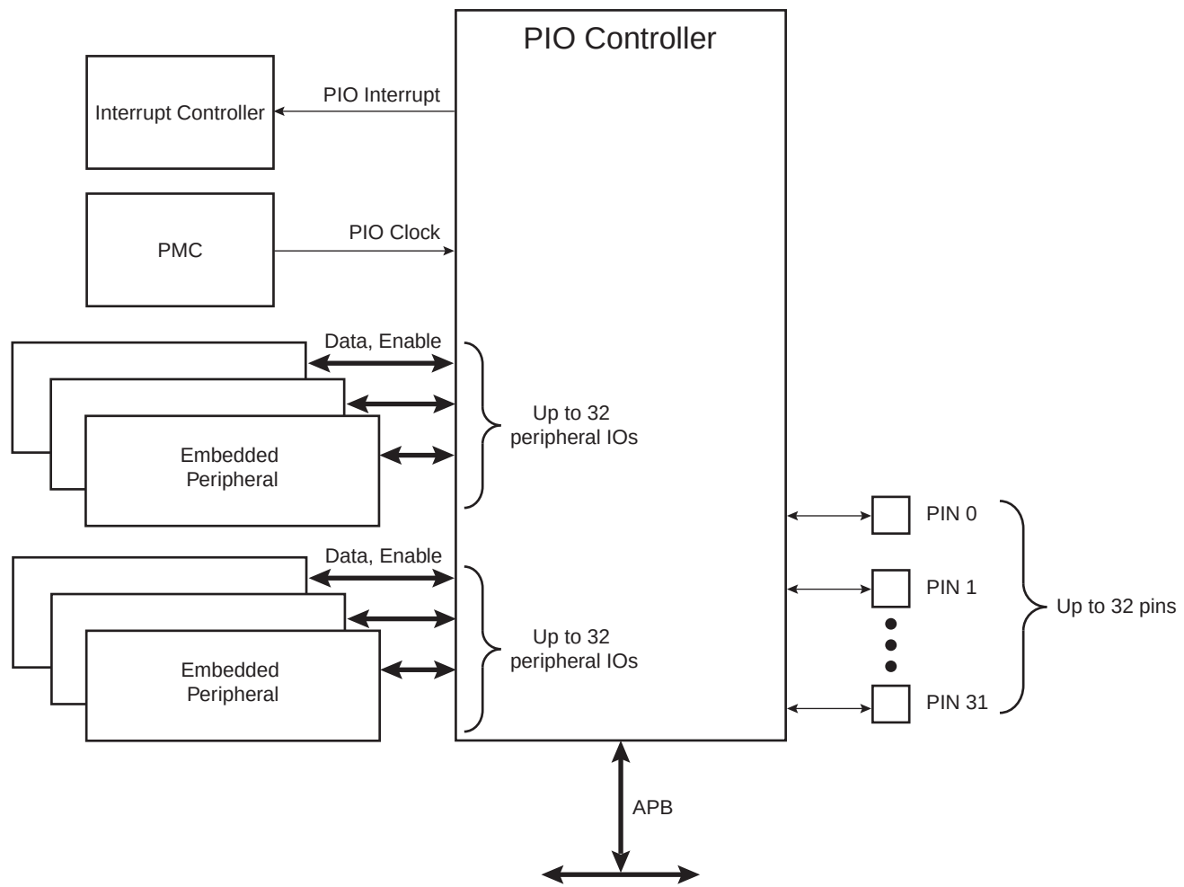
Figure 27-1. Block Diagram
