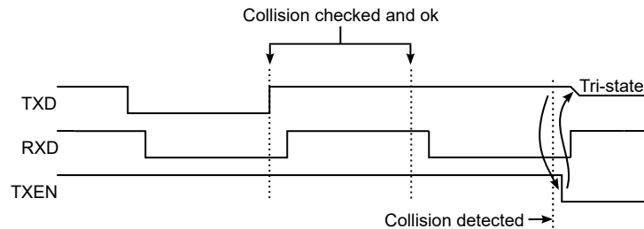
Figure 35-19. Collision Detected
