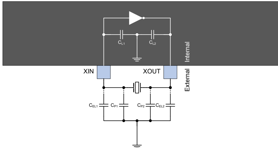
Figure 51-11. Crystal Circuit With Internal, External and Parasitic Capacitance
