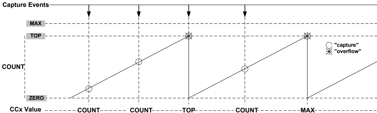
Figure 38-15. Time-Stamp
