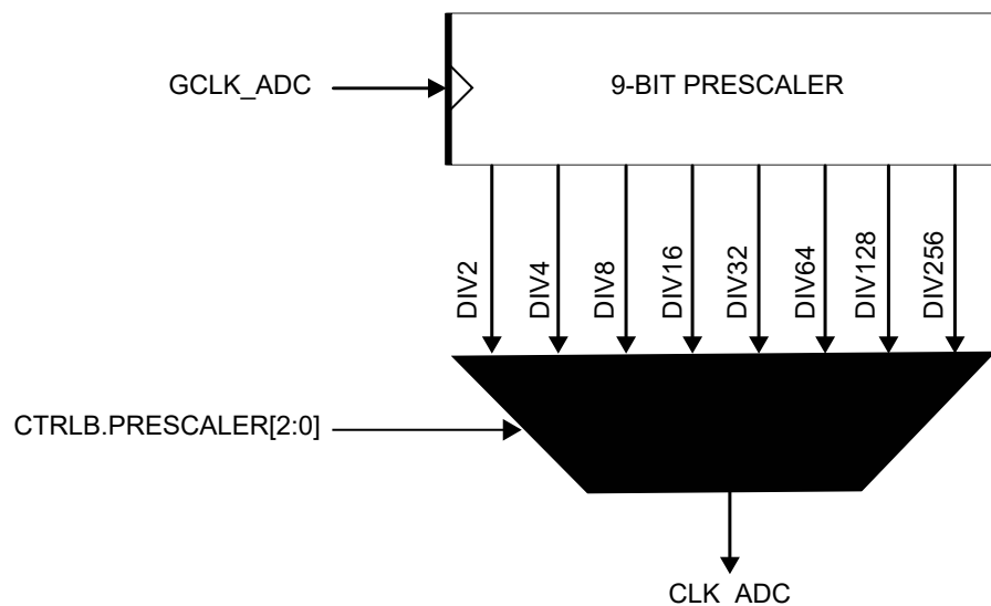
Figure 41-2. ADC Prescaler
