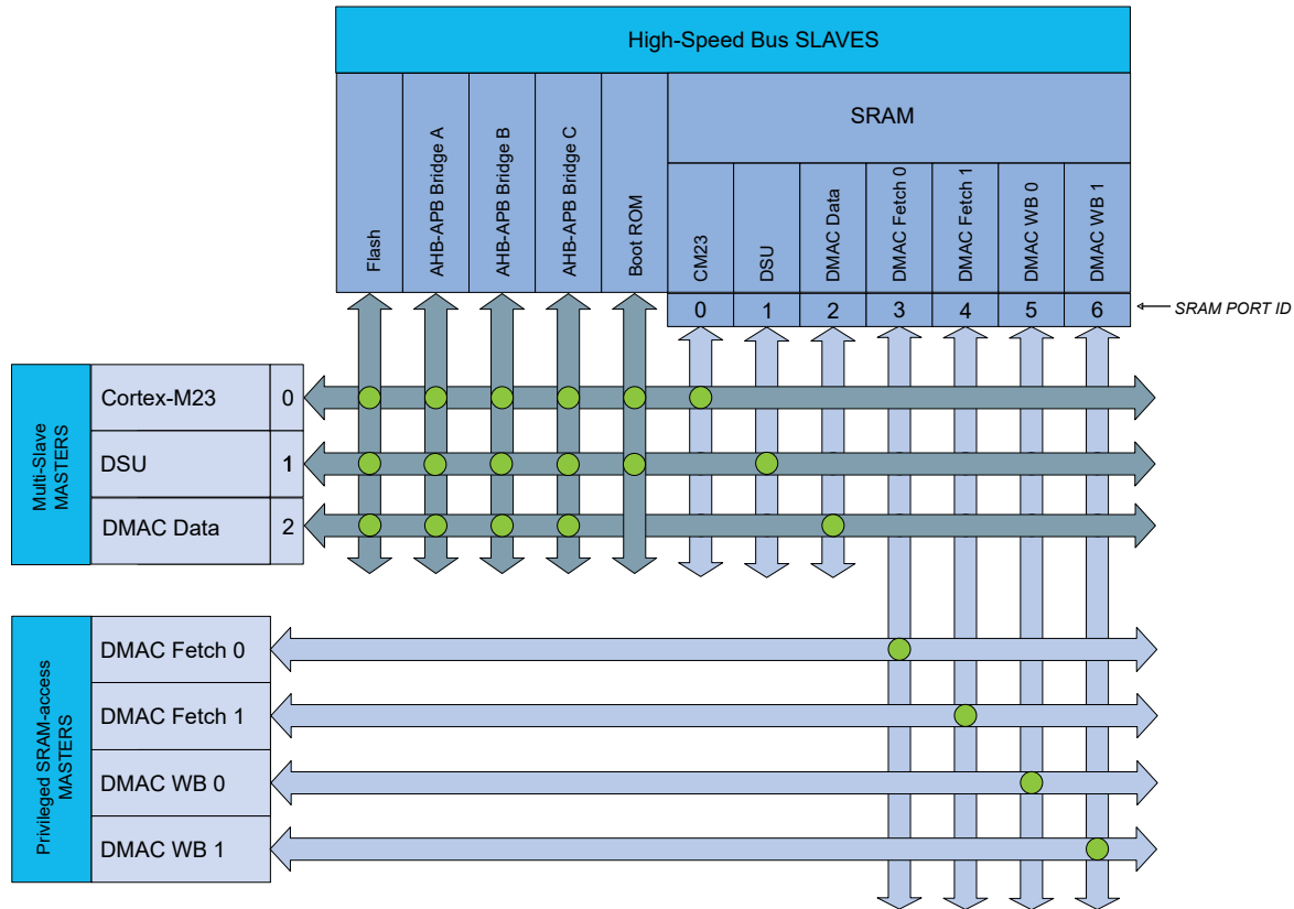
Figure 11-1. Master-to-Slave Access
