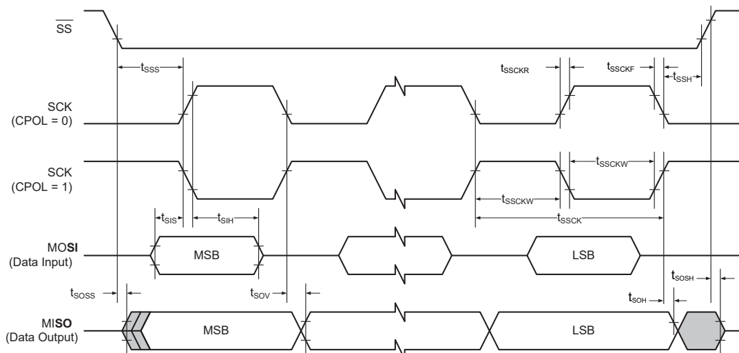
Figure 47-5. SPI Timing Requirements in Slave Mode
