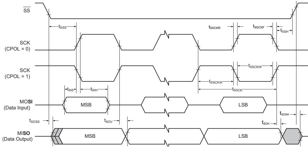
Figure 47-3. SPI Timing Requirements in Slave Mode
