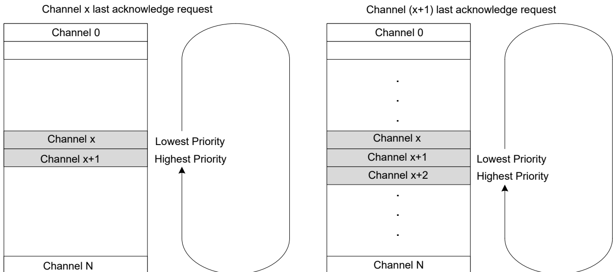
Figure 33-4. Round-Robin Scheduling
