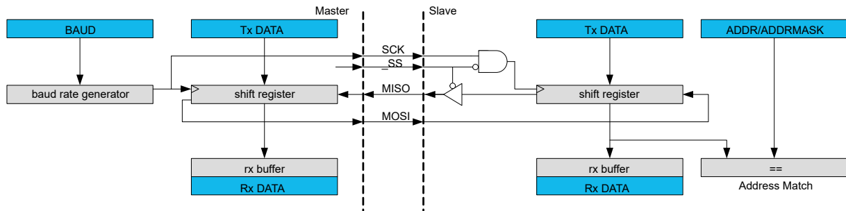
Figure 36-1. Full-Duplex SPI Master Slave Interconnection
