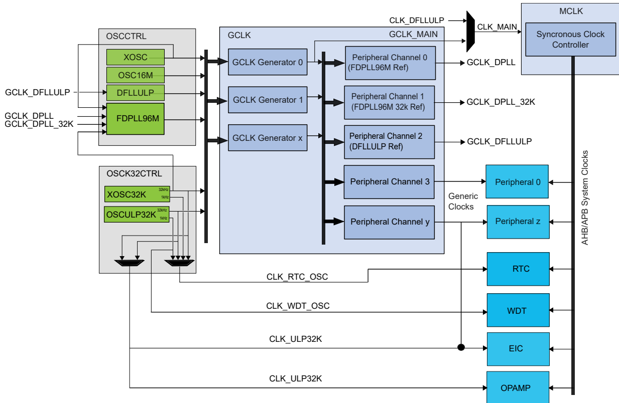
Figure 17-1. Clock Distribution
