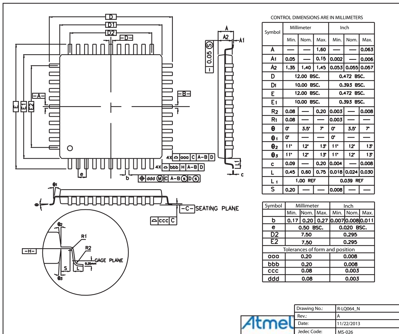
Figure 5-3. 64-lead LQFP Package Mechanical Drawing
