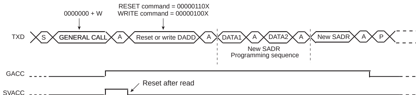
Figure 29-26. Master Performs a General Call
