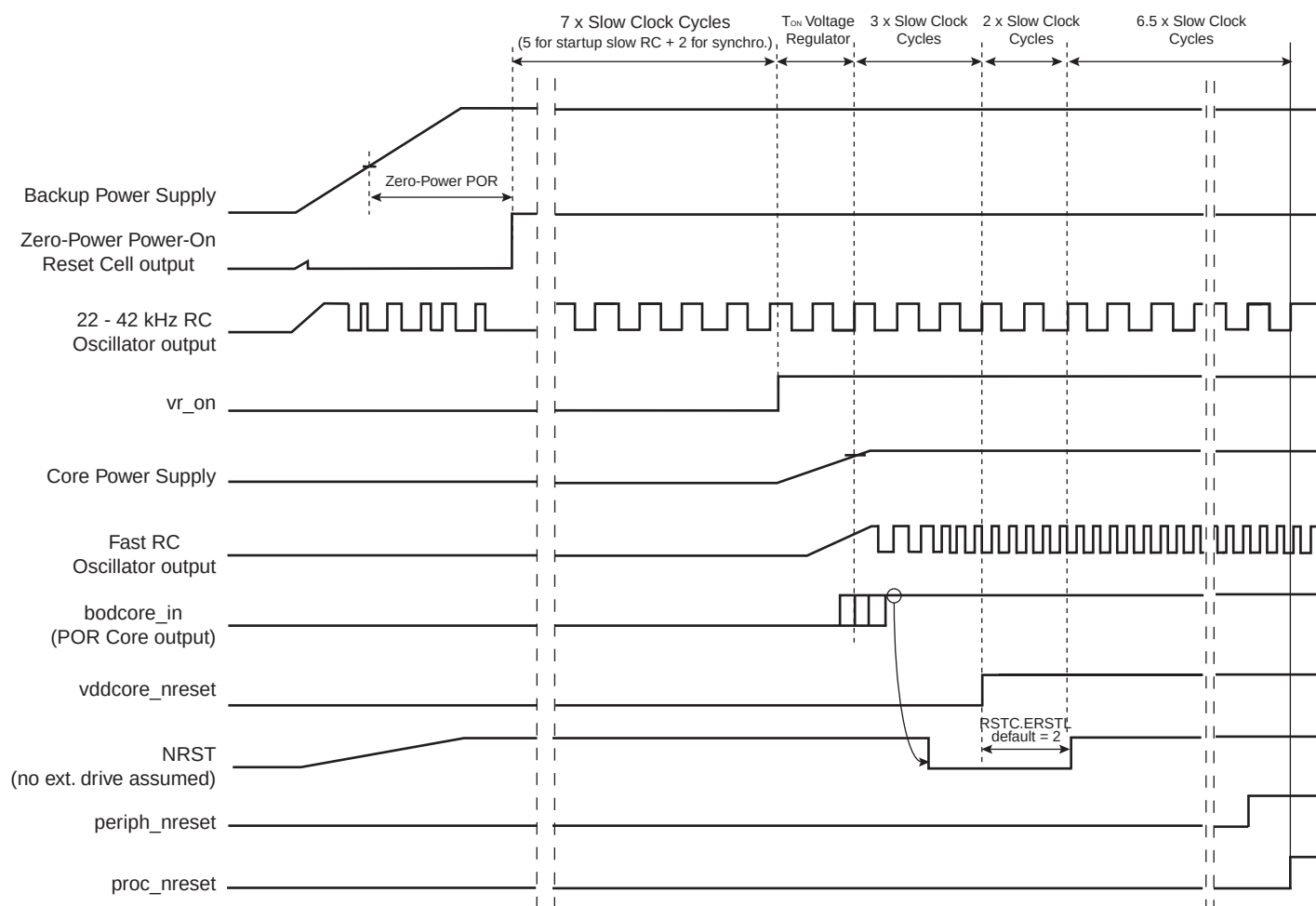
Figure 18-3. Raising the VDDIO Power Supply
