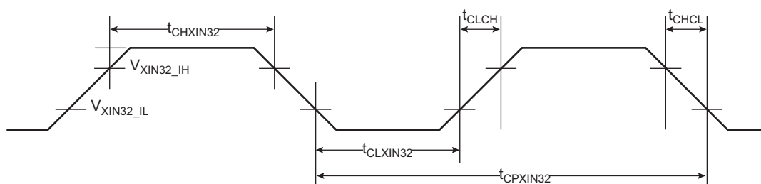
Figure 37-8. XIN32 Clock Timing
