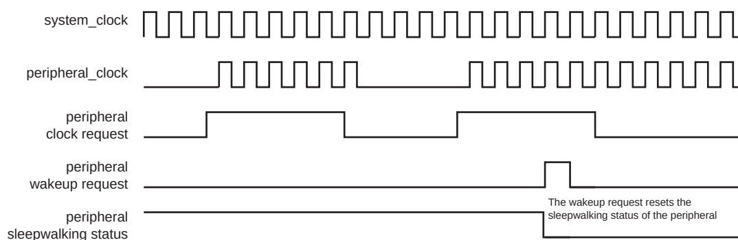
Figure 25-4. SleepWalking During Active Mode
