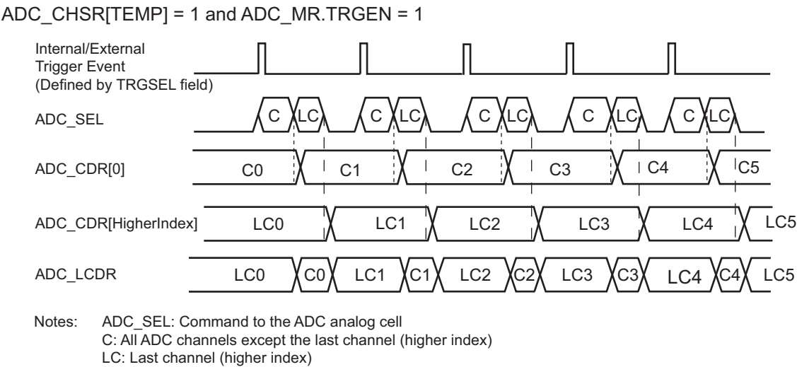
Figure 36-6. Same Trigger for All Channels
