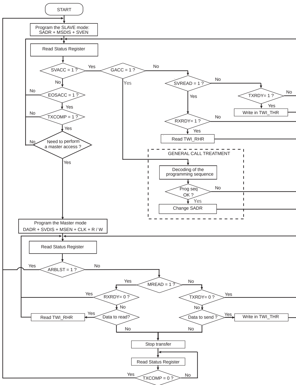
Figure 30-21. Multi-master Flowchart
