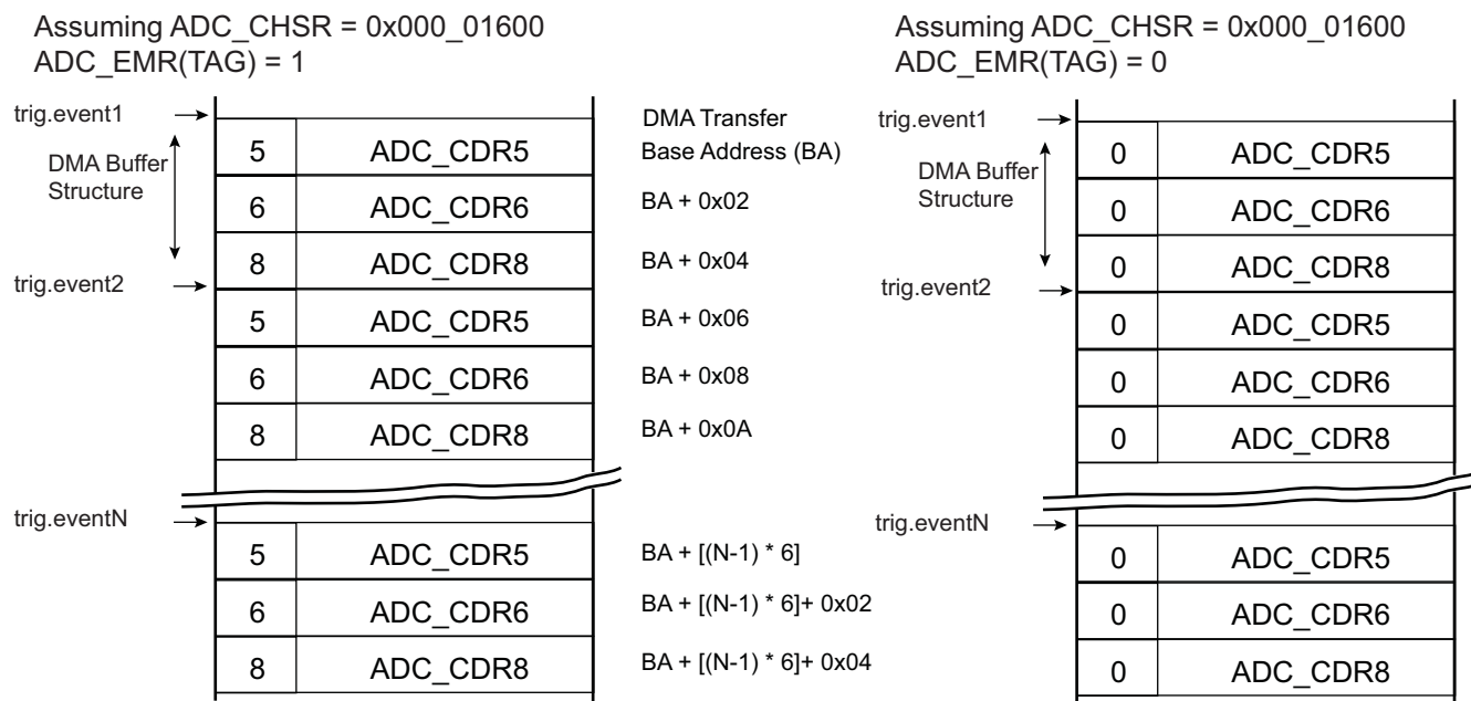
Figure 36-12. Buffer Structure
