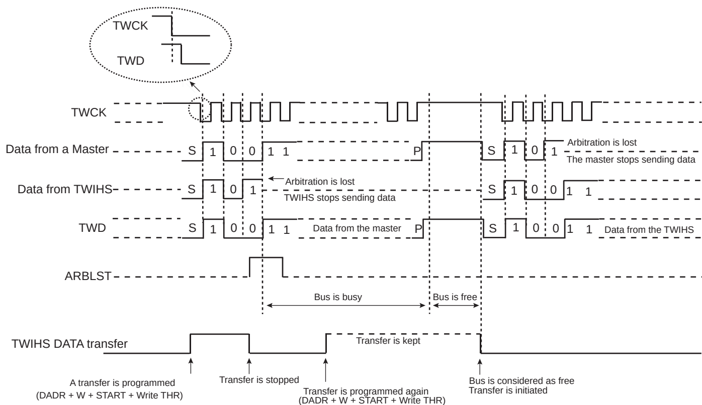
Figure 29-22. Arbitration Cases
