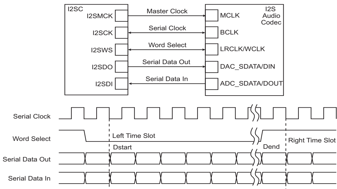
Figure 31-7. Codec Application Block Diagram
