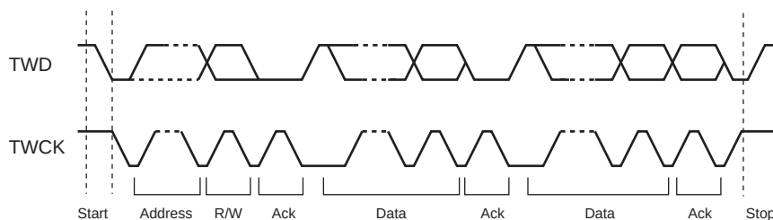
Figure 30-3. Transfer Format
