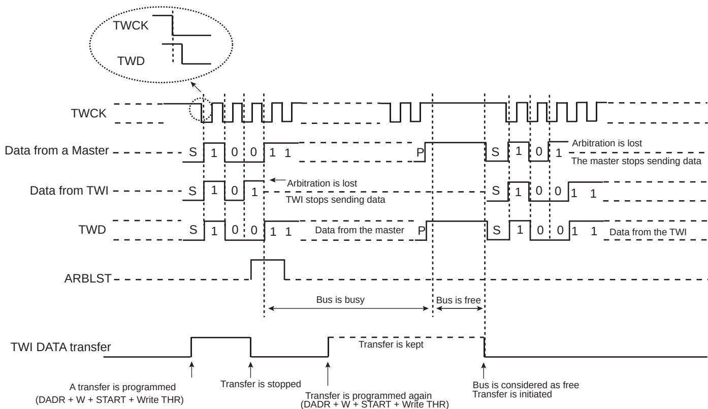
Figure 30-20. Arbitration Cases
