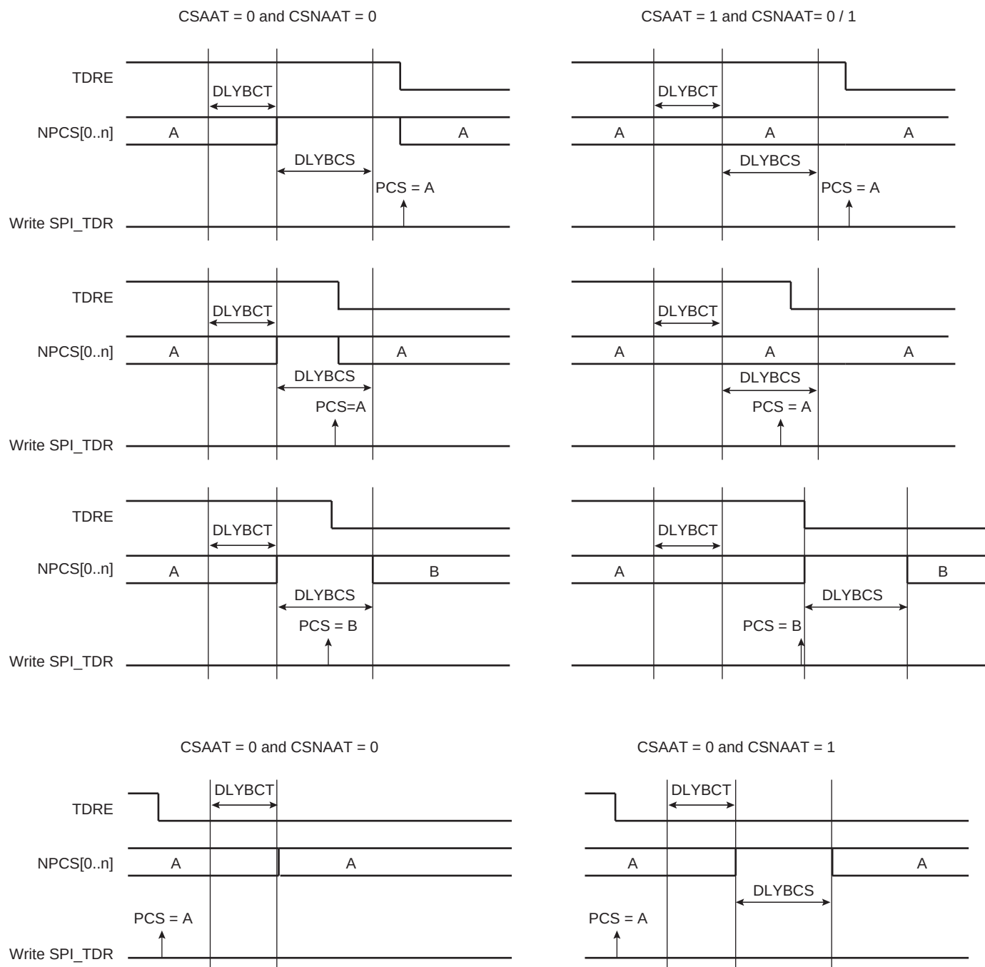
Figure 28-12. Peripheral Deselection
