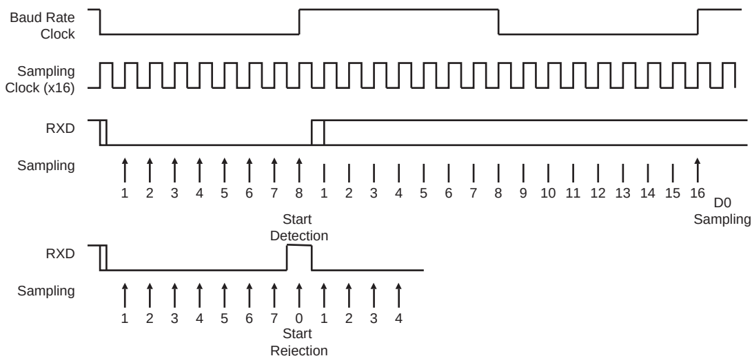
Figure 33-7. Asynchronous Start Detection
