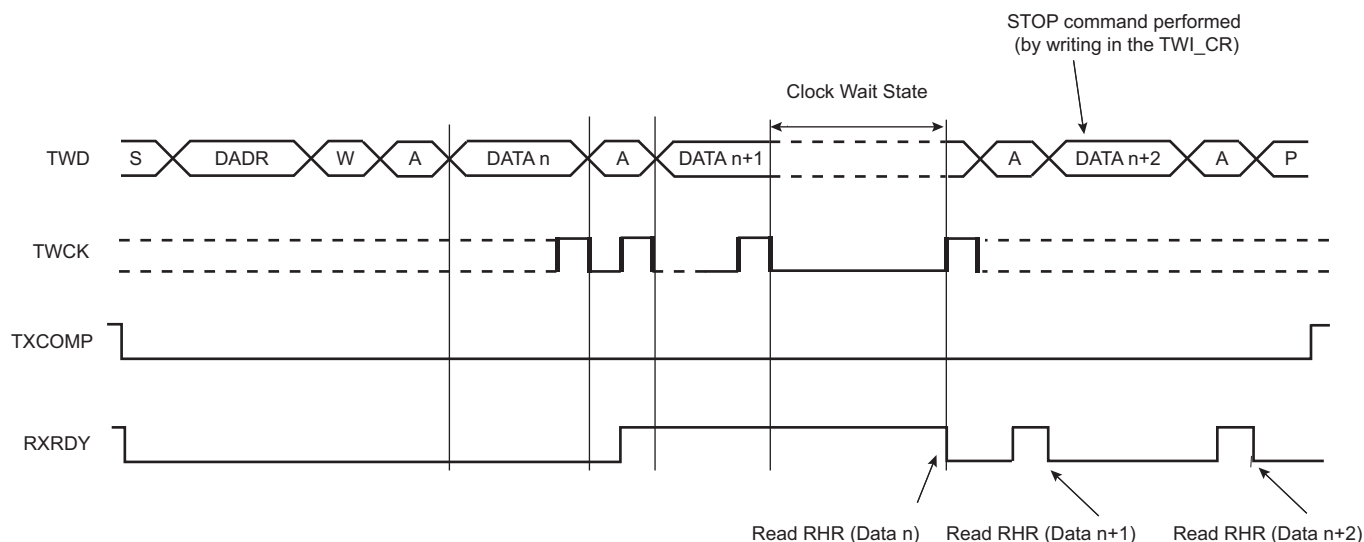
Figure 30-9. Master Read Wait State with Multiple Data Bytes
