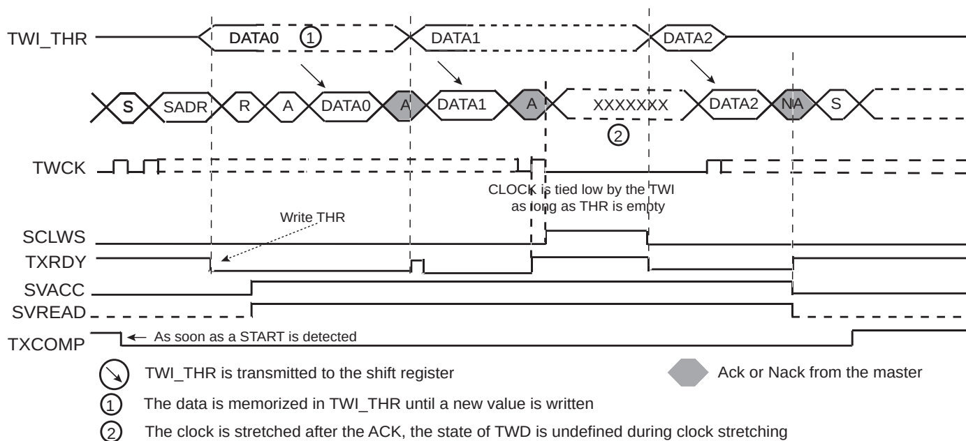
Figure 30-25. Clock Stretching in Read Mode
