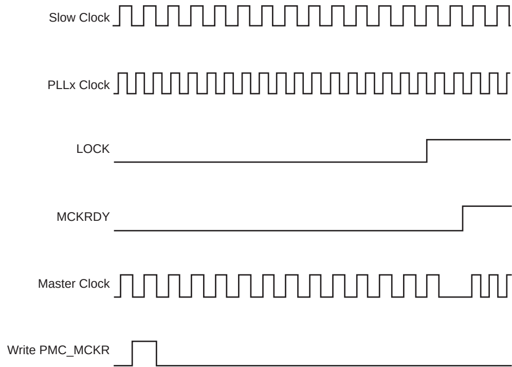
Figure 25-7. Switch Master Clock from Slow Clock to PLLx Clock
