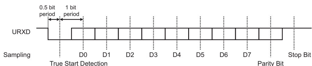
Figure 34-4. Character Reception
