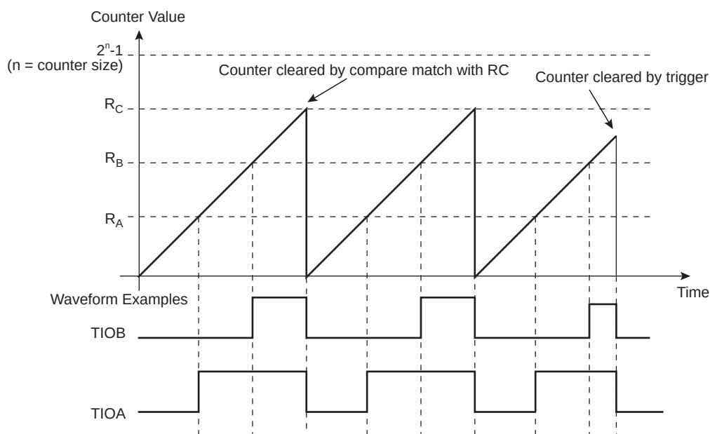
Figure 35-11. WAVSEL = 10 with Trigger
