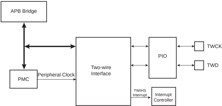
Figure 29-1. Block Diagram
