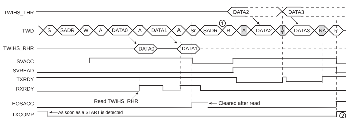
Figure 29-30. Repeated Start and Reversal from Write Mode to Read Mode
