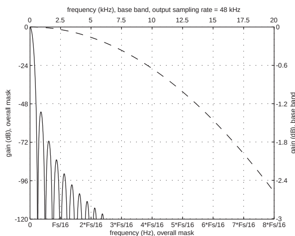
Figure 32-4. Spectral Mask of an OSR = 64, F_s = 3.072 MHz, Fourth-order Sinc Filter: Overall Response (continuous line) and 0 to 20 kHz Bandwidth Response (dashed line)
