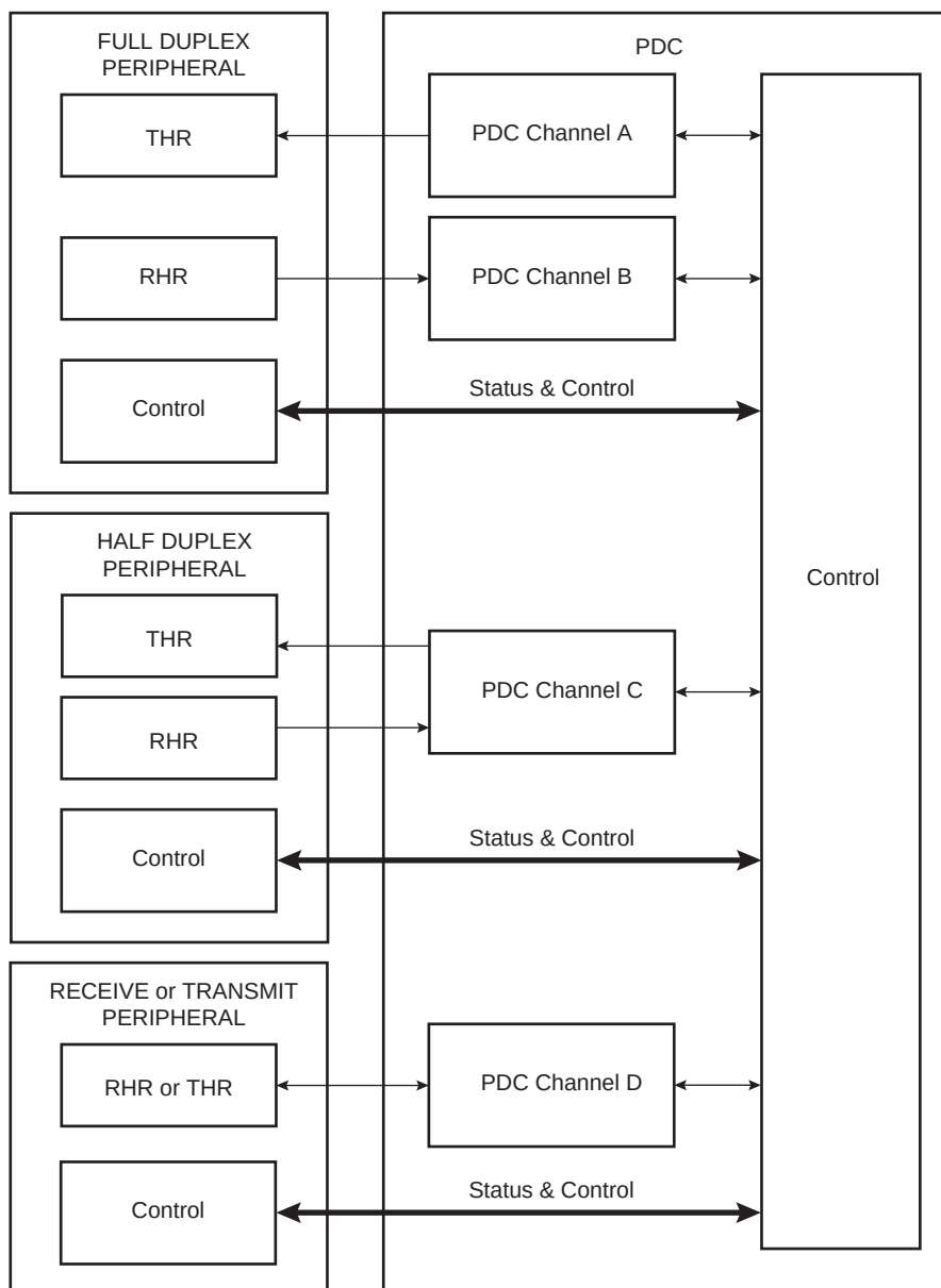
Figure 23-1. Block Diagram
