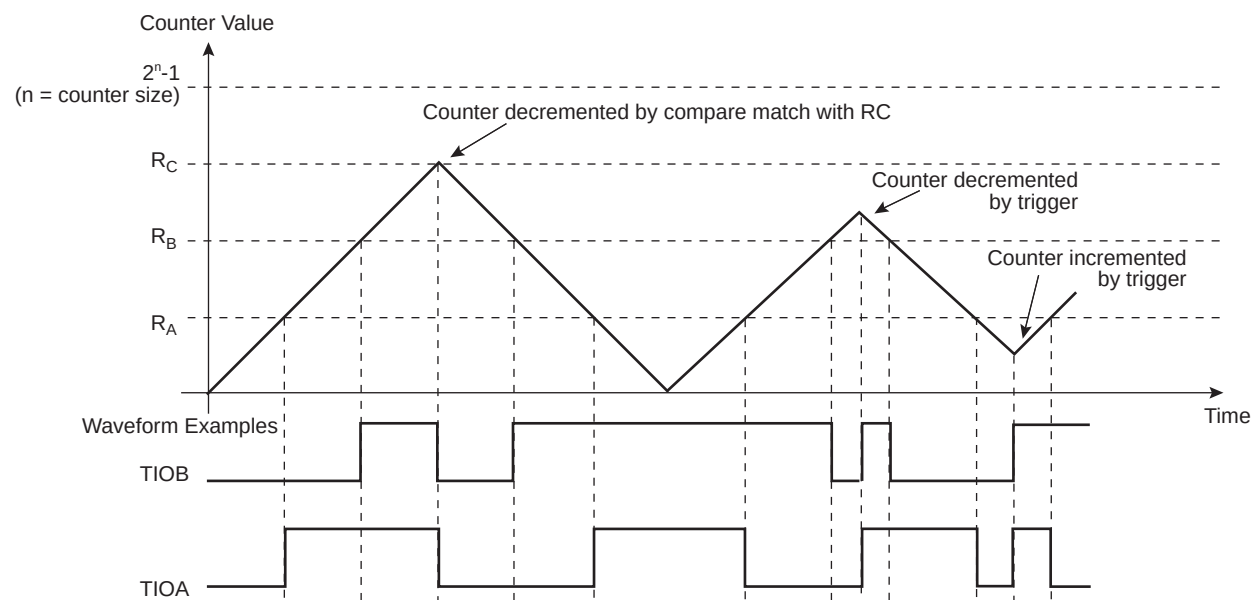
Figure 35-15. WAVSEL = 11 with Trigger
