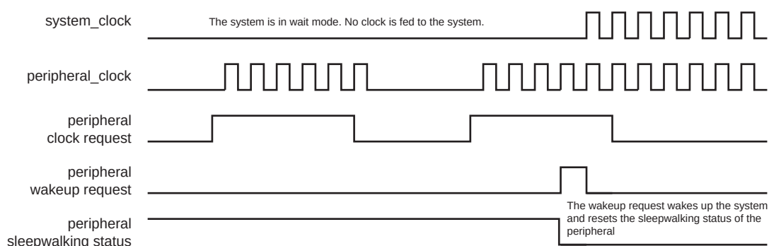
Figure 25-3. SleepWalking During Wait Mode
