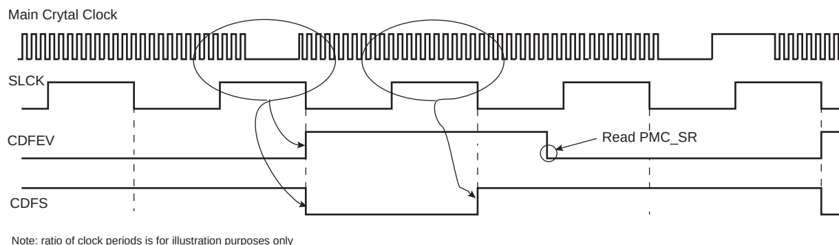
Figure 25-6. Clock Failure Detection (Example)
