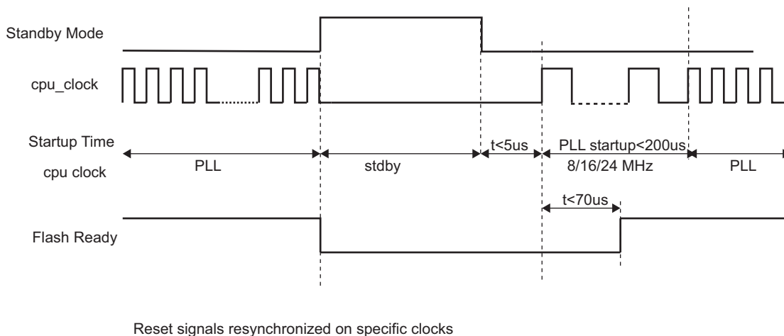
Figure 5-2. Start-up Sequence
