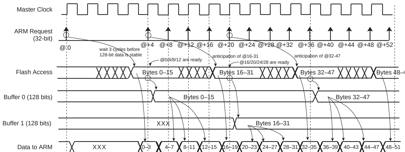
Figure 21-4. Code Read Optimization for FWS = 3
