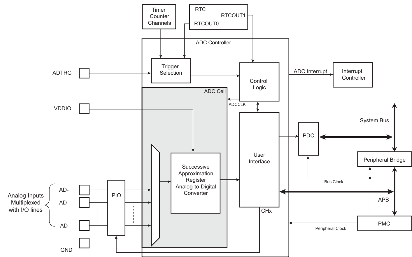
Figure 36-1. Analog-to-Digital Converter Block Diagram
