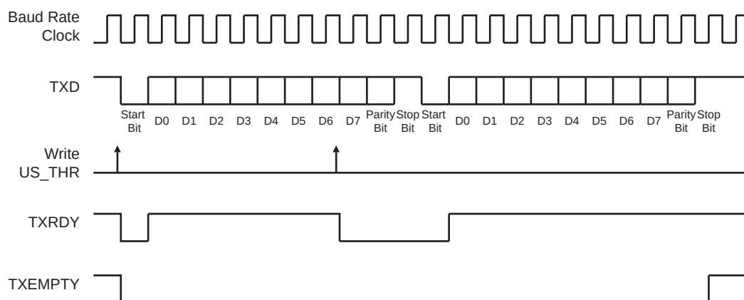
Figure 33-6. Transmitter Status
