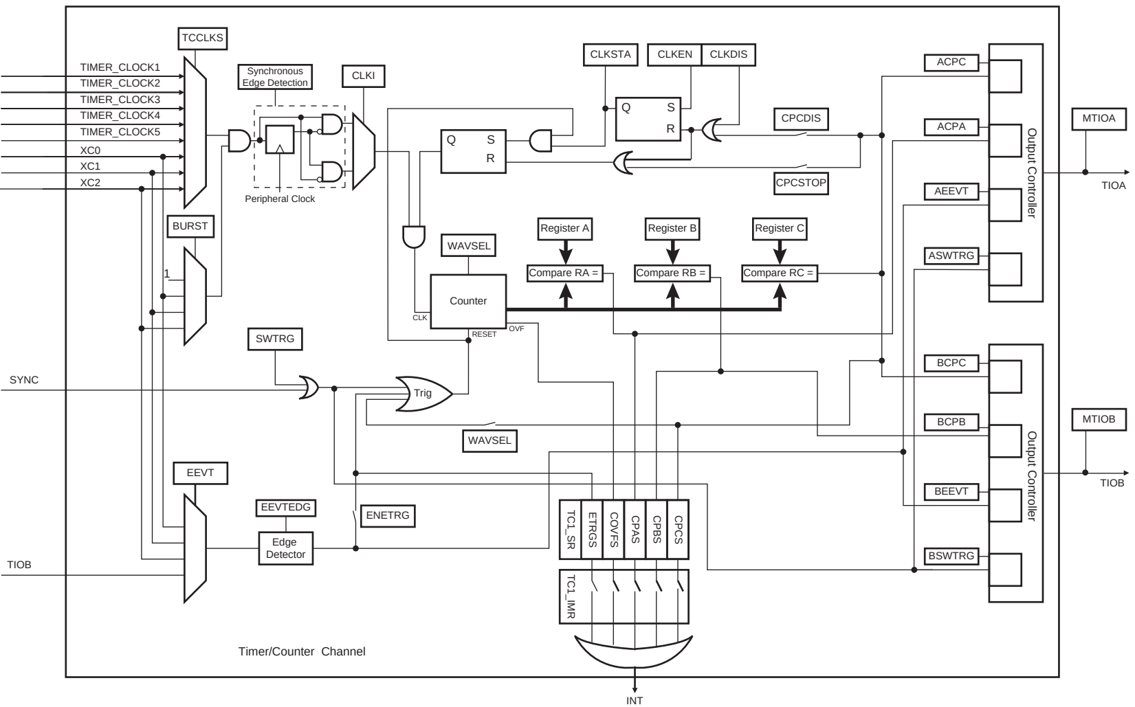
Figure 35-7. Waveform Mode
