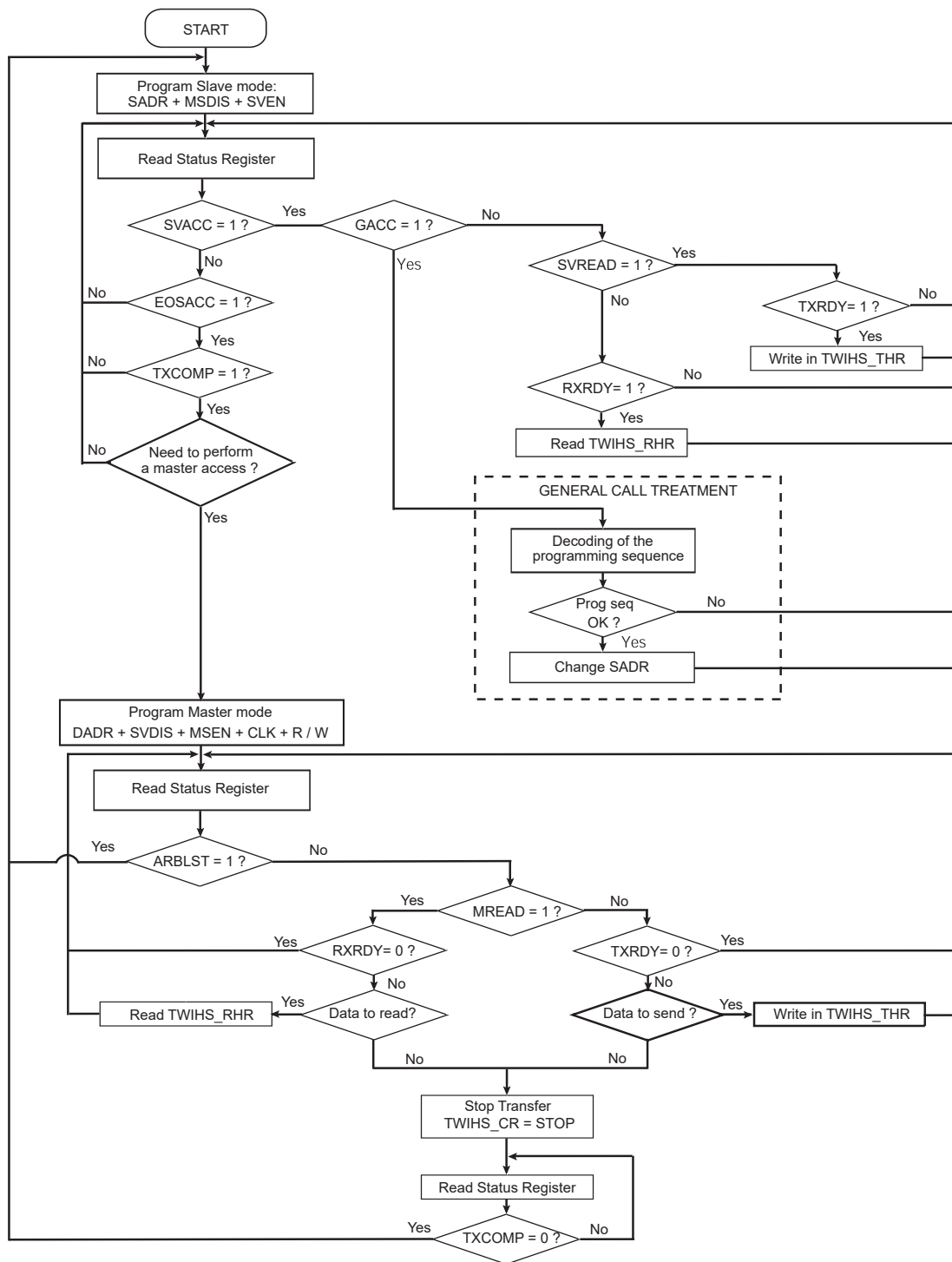
Figure 43-30. Multimaster Flowchart
