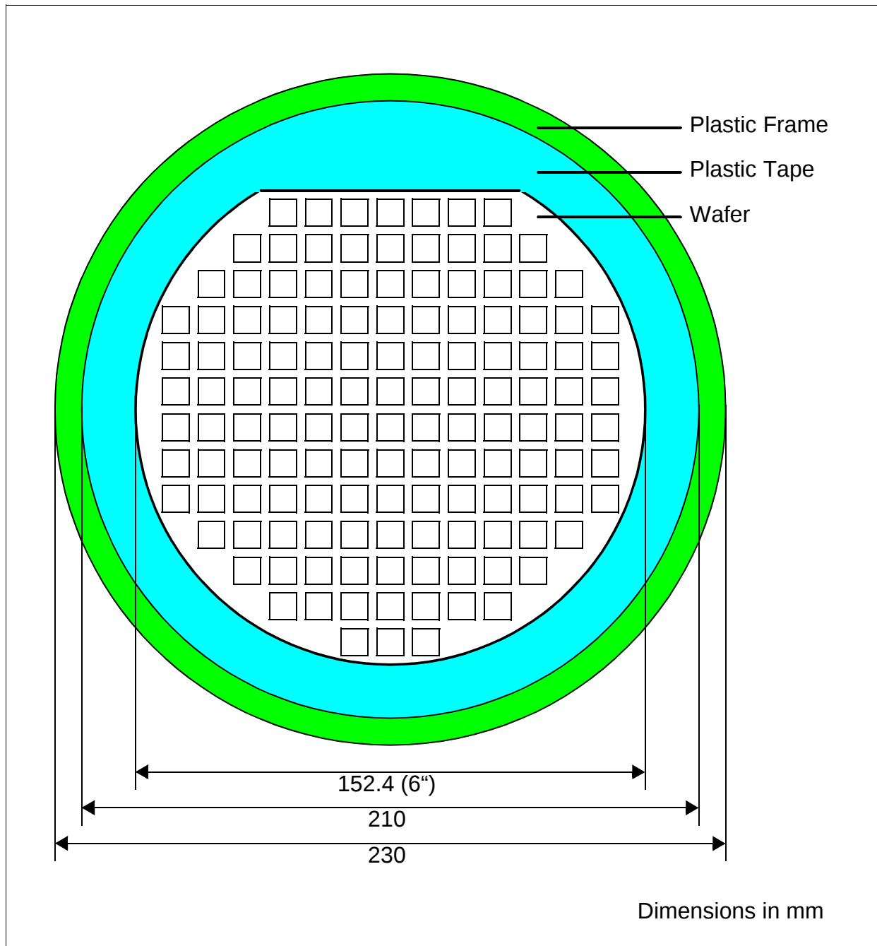
Figure 6 Wafer Outline
