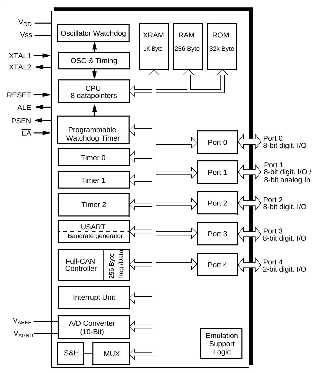
Figure 4 Block Diagram
