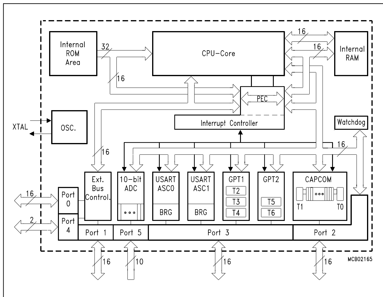
Figure 3 Block Diagram
