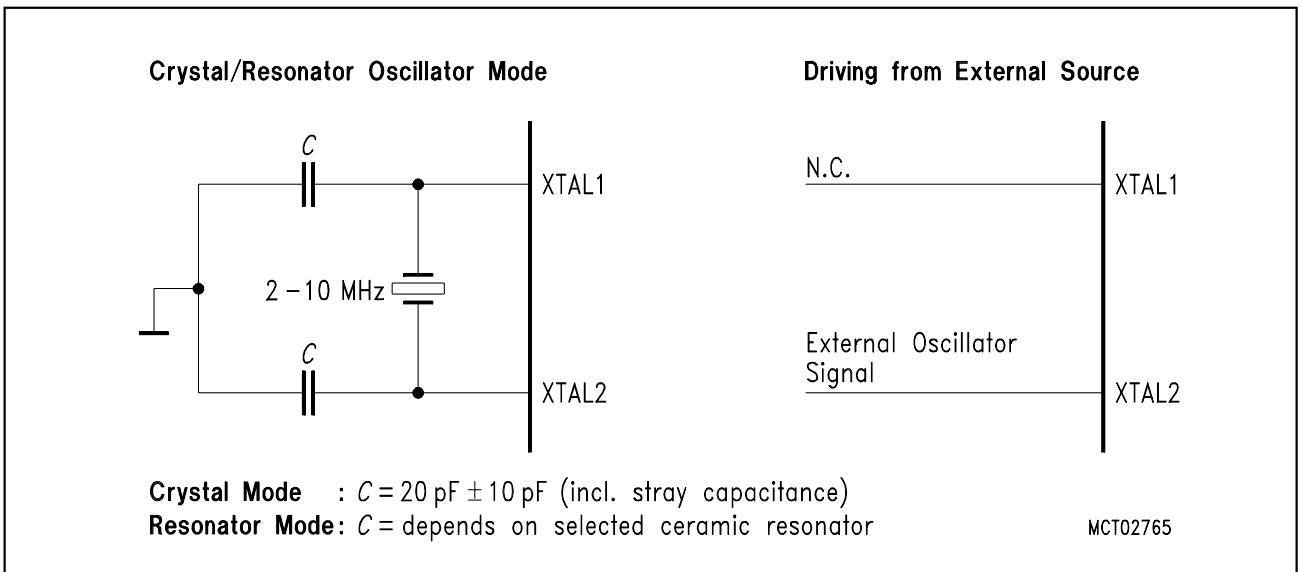
Figure 35 Recommended Oscillator Circuits for Crystal Oscillator
