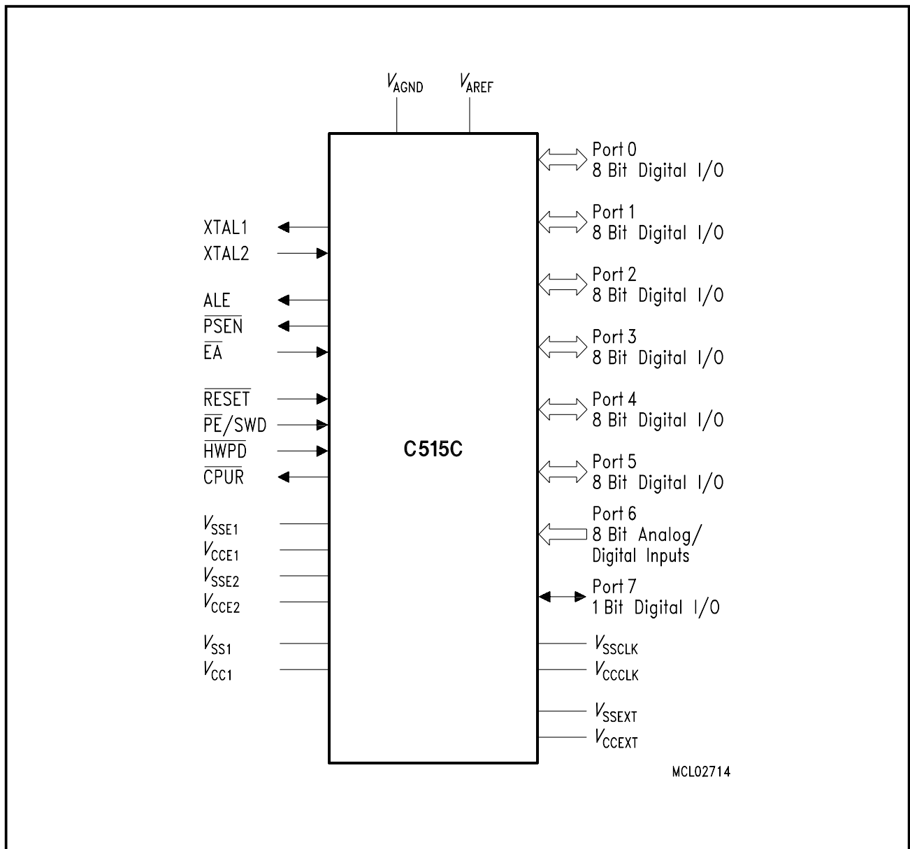
Figure 2 Logic Symbol
