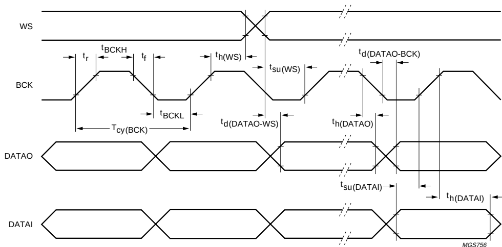
Fig.2 Serial interface input data timing.
