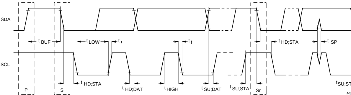
Fig.5 Timing of the I²C-bus transfer.
