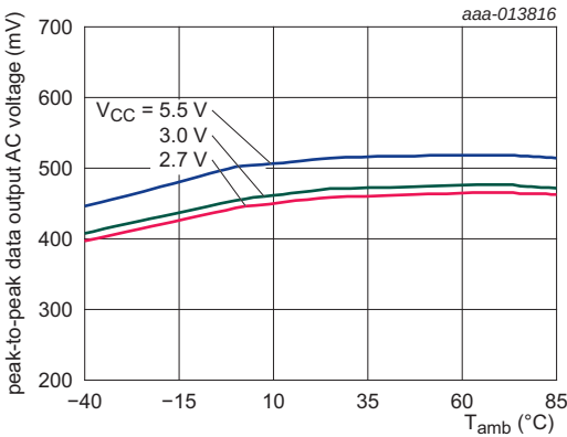
Fig 14. Data output AC voltage versus ambient temperature
