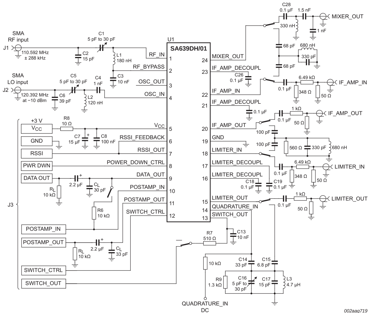
Fig 25. SA639 test circuit
