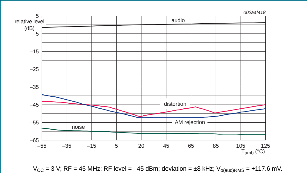
Fig 12. Relative audio level, distortion, AM rejection and noise versus ambient temperature
