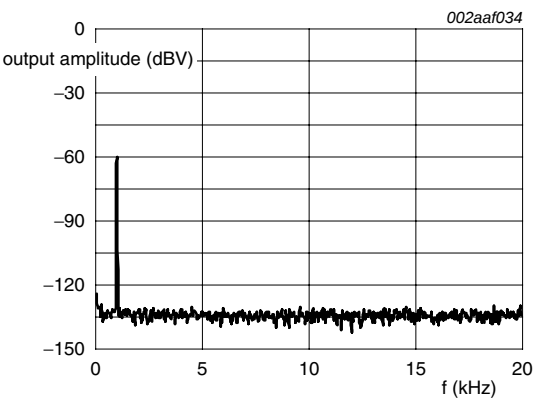
Fig 18. Output amplitude versus frequency
