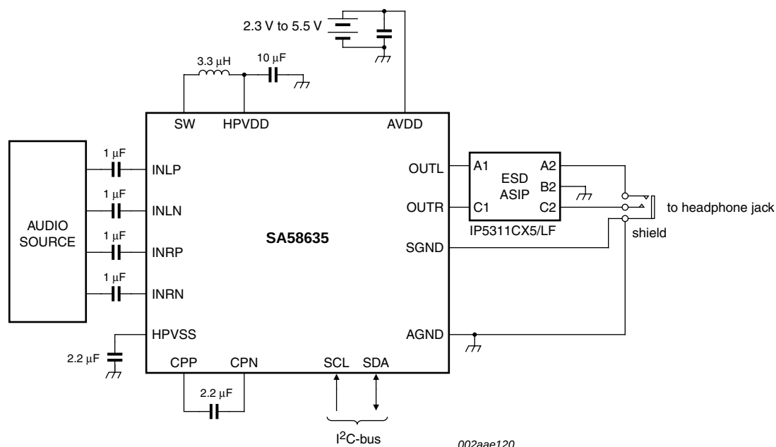
Fig 25. Typical application
