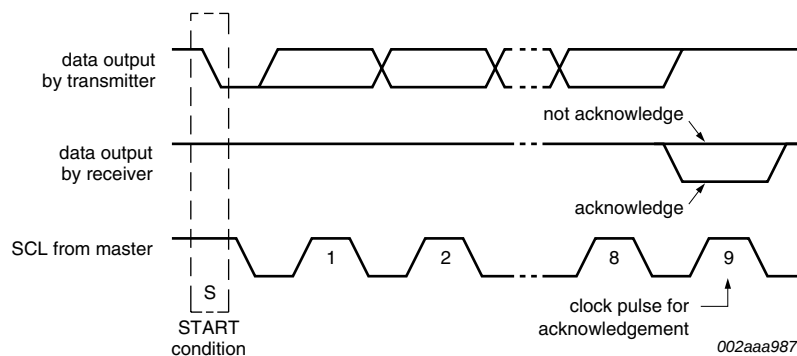
Fig 7. Acknowledgement on the I 2 C-bus
