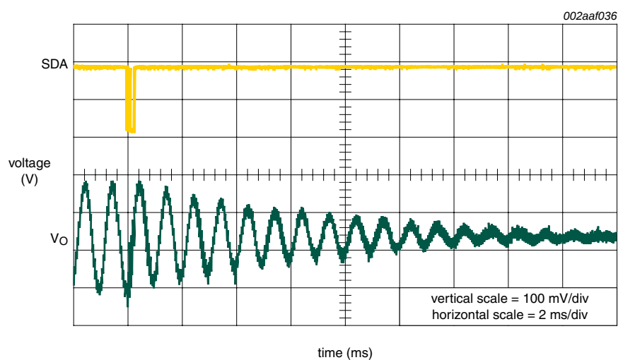
Fig 23. Start-up waveform
