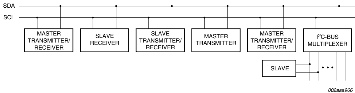
Fig 6. System configuration
