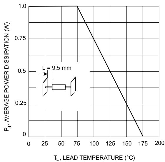
Fig. 5, Power Derating
