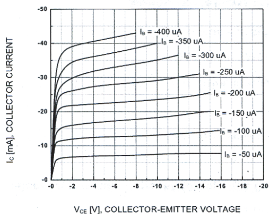
FIG.1 Static Characteristic
