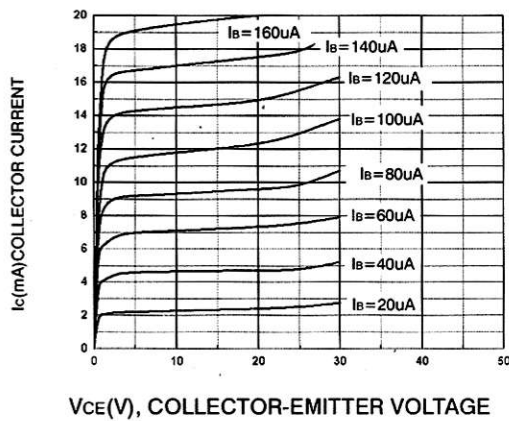
Static Characteristic
