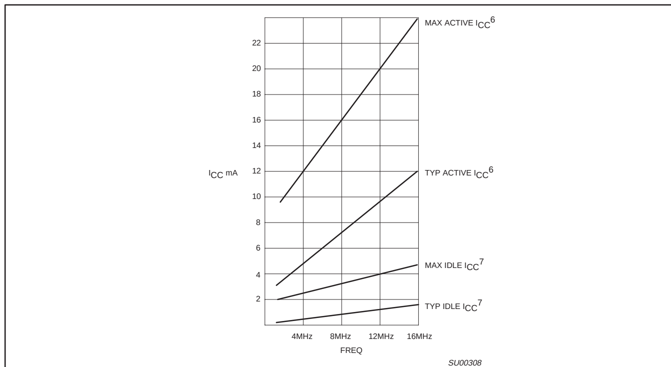
Figure 6. I_{CC} vs. FREQ Maximum I_{CC} values taken at V_{CC} = 5.5V and worst case temperature. Typical I_{CC} values taken at V_{CC} = 5.0 V and 25^{\circ}C . Notes 6 and 7 refer to AC Electrical Characteristics.
