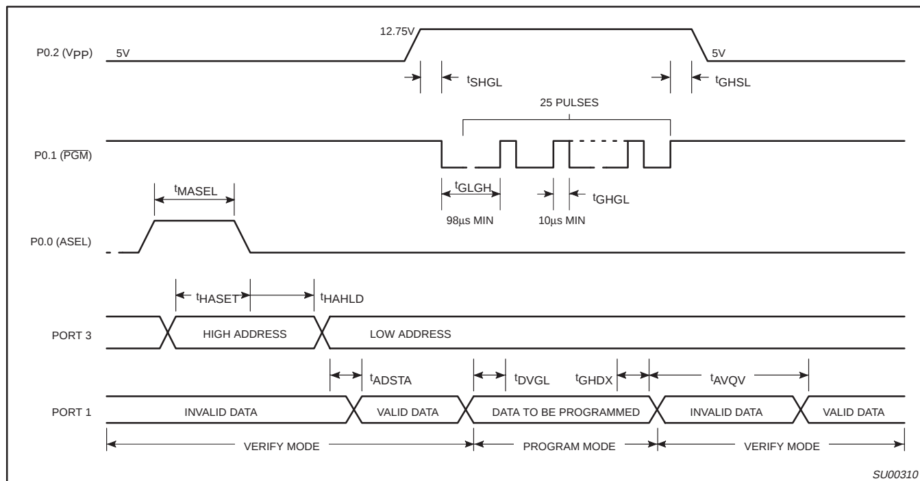
Figure 9. Program/Verify Cycle
