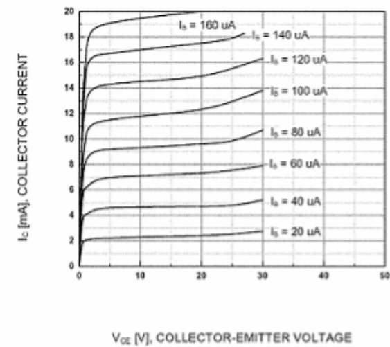
Static Characteristic
