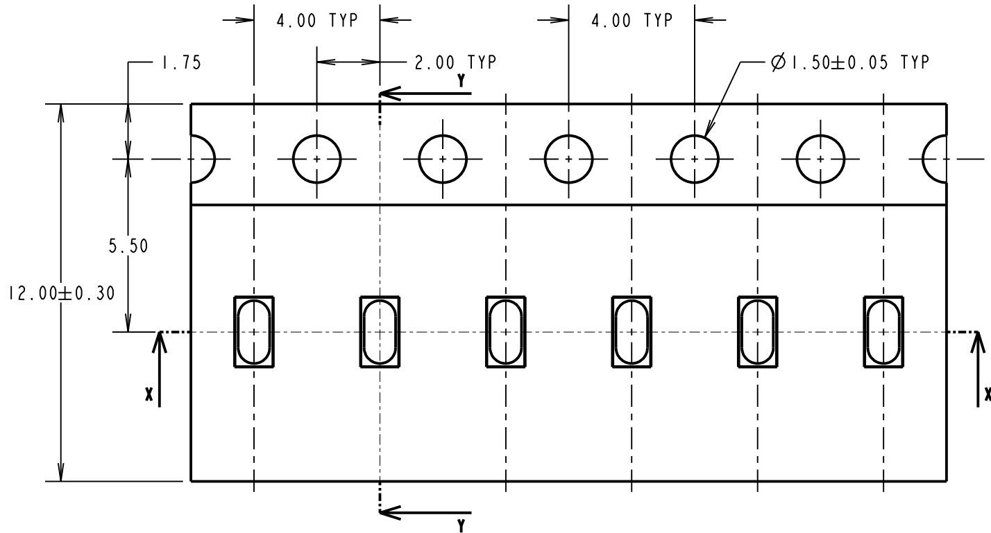
SECTION X-X
