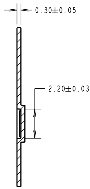
SECTION Y-Y
