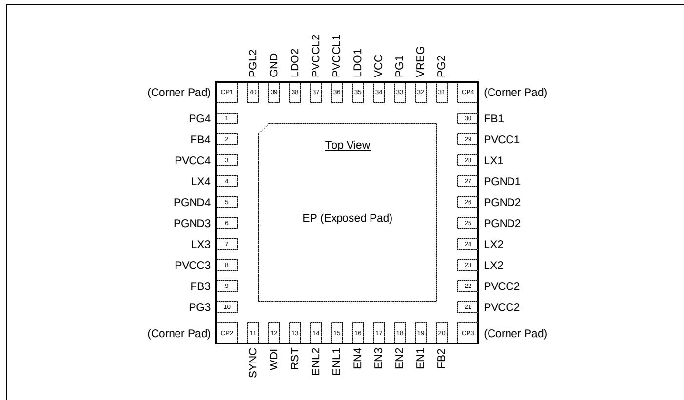
Figure 2-1 Pin Configuration
