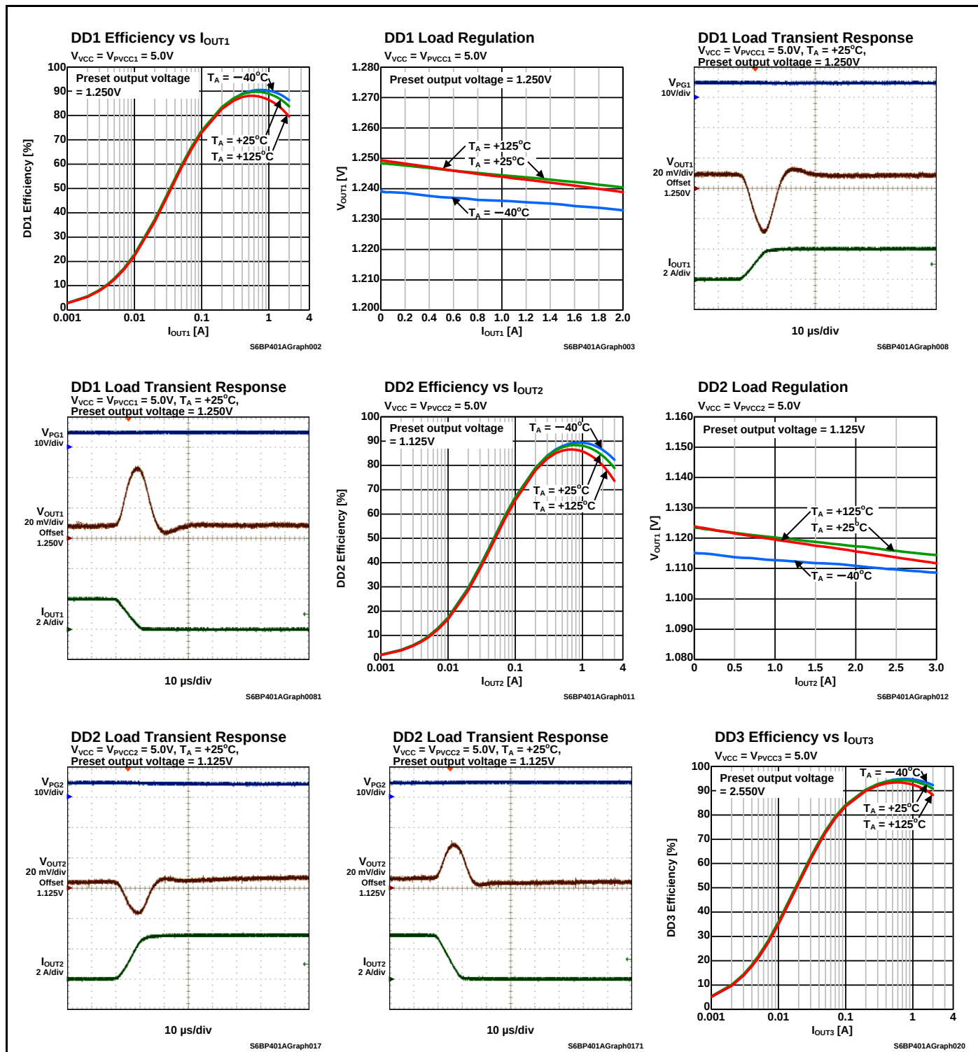
Figure 12-1 DC/DC Converter
