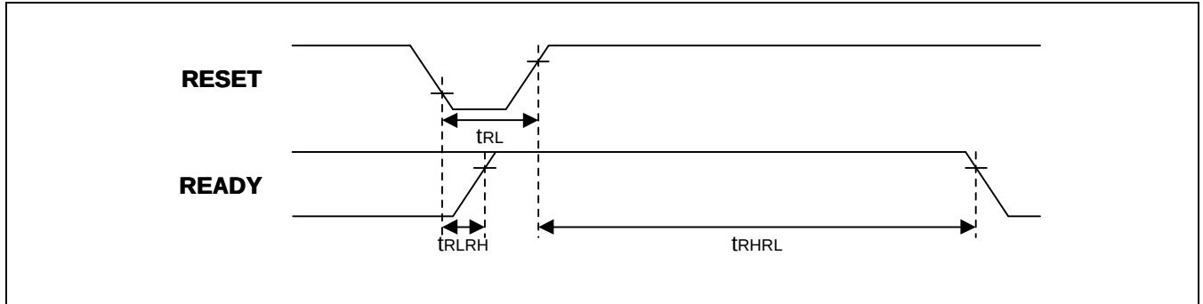
Figure 17: Reset Timing
