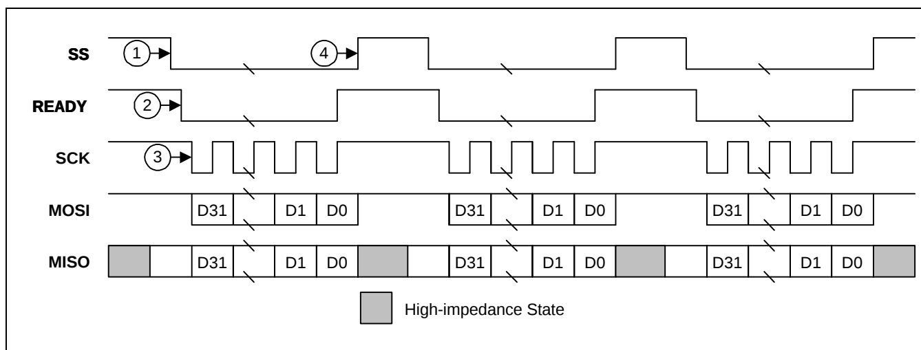
Figure 6: Typical Multiple Packet Communications Initiated by the Host
