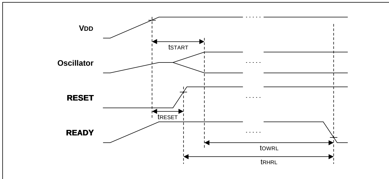
Figure 16: Start-up Timing
