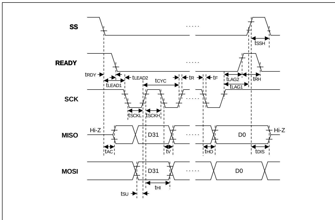
Figure 15: SPI Timing
