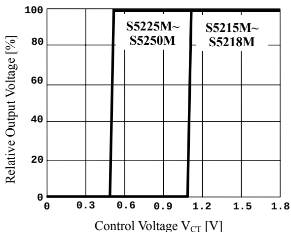
Fig.3 V_O vs. V_{CT}
