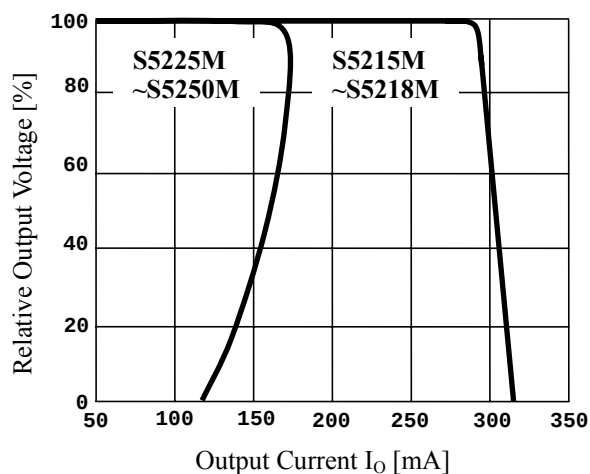
Fig.2 V_O vs. I_O
