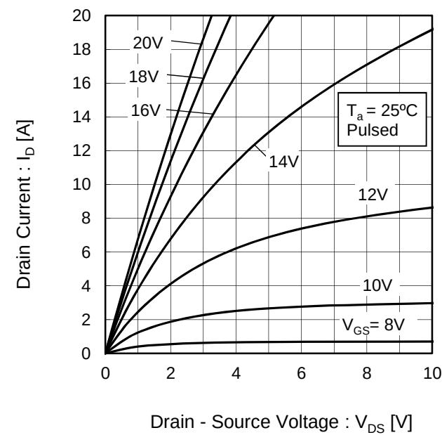
Fig.1 Typical Output Characteristics(I)
