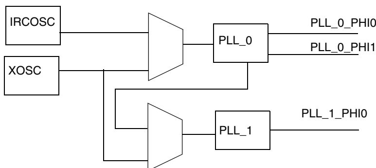
Figure 6. PLL integration
