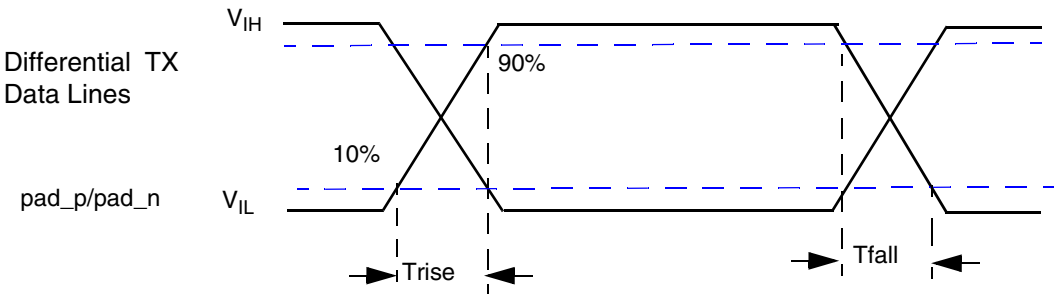
Figure 23. Rise/fall time
