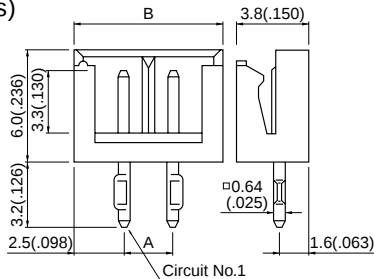
(3 to 15 circuits)
