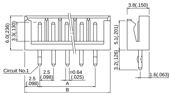
(3 to 15 circuits)
