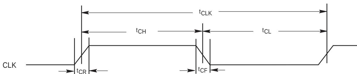
Figure II.6. CLK Characterization
