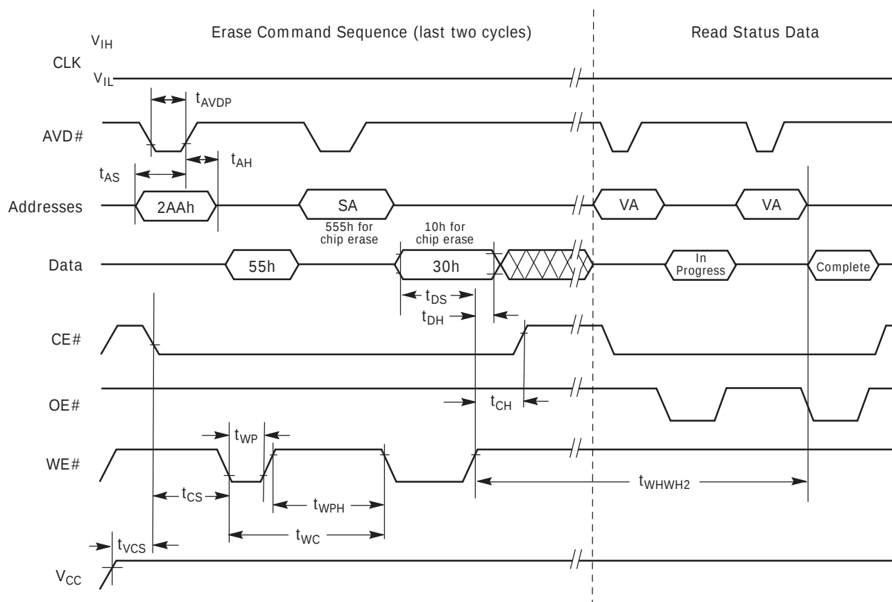
Figure II.I3. Chip/Sector Erase Operation Timings
