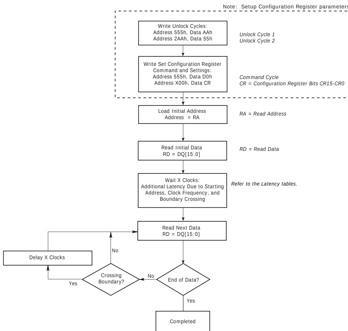
Figure 7.2. Synchronous Read
