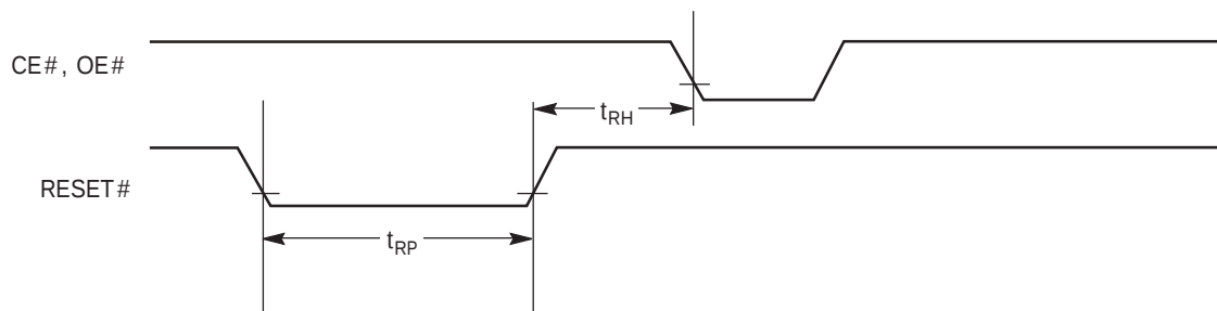
Figure II.I2. Reset Timings
