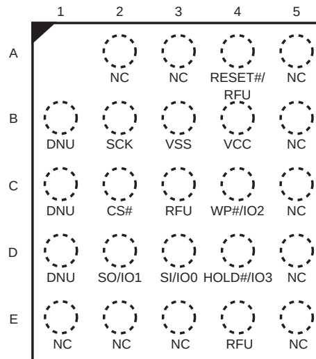
Figure 40. 24-Ball BGA, 5 x 5 Ball Footprint (FAB024), Top View [31]
