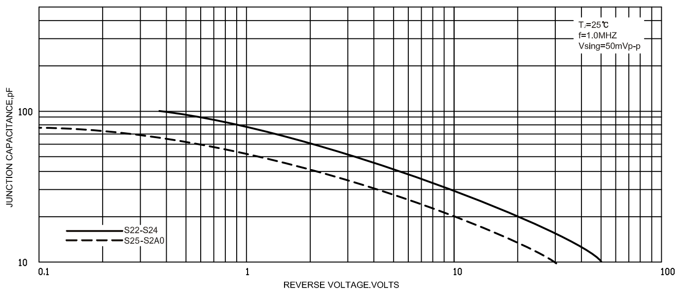
FIG.5-TYPICAL JUNCTION CAPACITANCE
