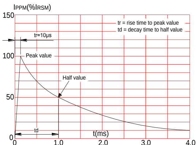
FIG.3: Pulse waveform
