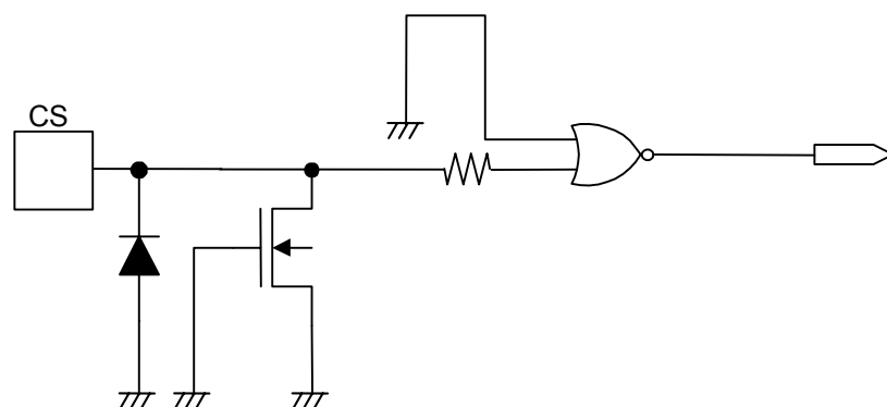
Figure 23 CS Pin
