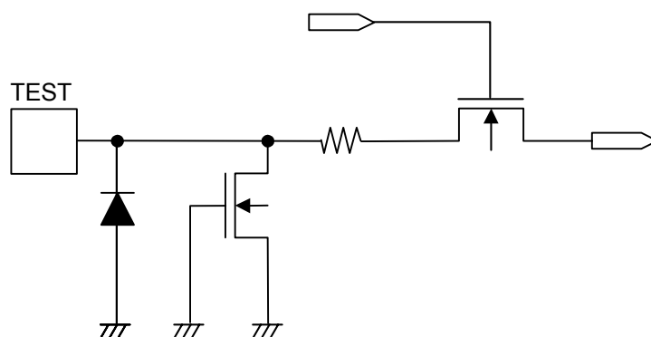
Figure 25 TEST Pin
