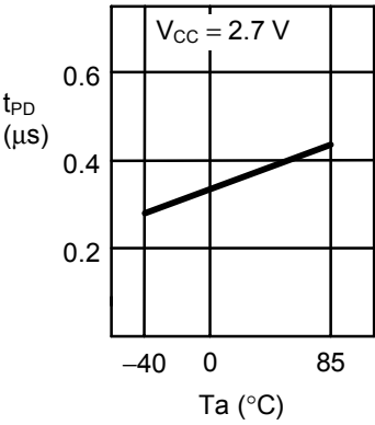
2. 7 Data output delay time t_{PD} vs. ambient temperature T_a
