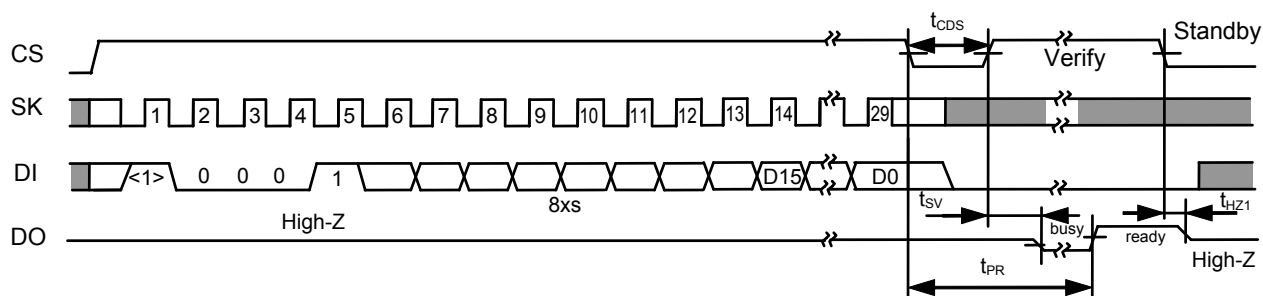
Figure 13 Chip Write Timing (S-93C76C/86C)
