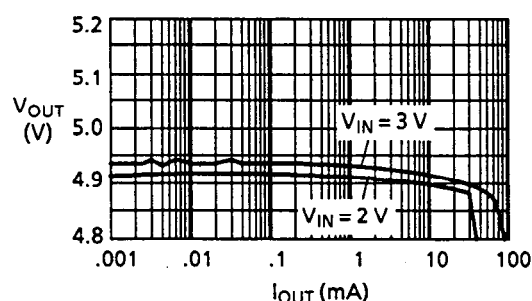
(a) I_{\text{OUT}}\text{-}V_{\text{OUT}}
