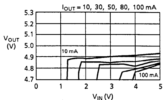
(b) V_{\text{IN}}\text{-}V_{\text{OUT}}
