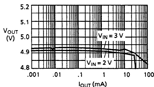
(a) I_{\text{OUT}}\text{-}V_{\text{OUT}}
