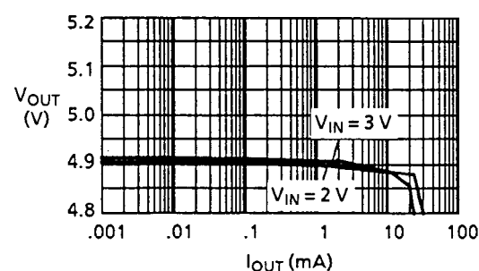
(a) I_{\text{OUT}}\text{-}V_{\text{OUT}}
