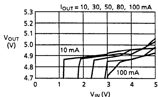
(b) V_{\text{IN}}\text{-}V_{\text{OUT}}
