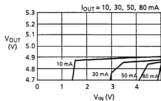
(b) V_{\text{IN}}\text{-}V_{\text{OUT}}
