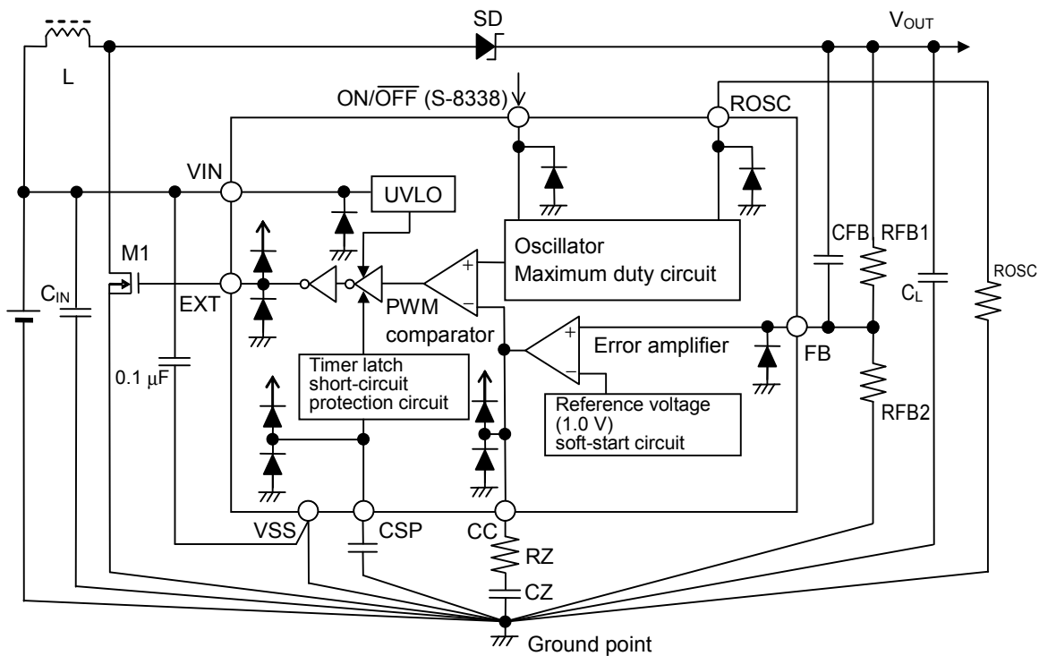
Figure 16 Standard Circuit (S-8338 Series)
