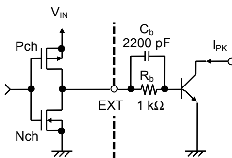
Figure 11 External Transistor Periphery
