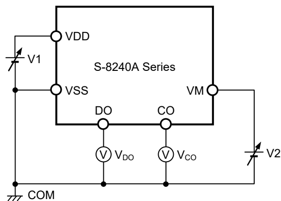
Figure 7 Test Circuit 2
