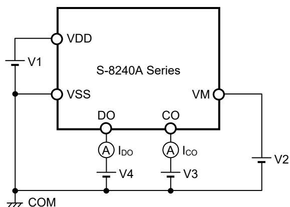
Figure 9 Test Circuit 4
