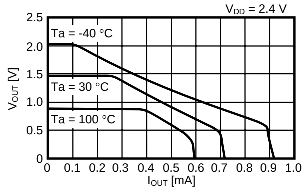
Load current ( I_{OUT} ) vs. Output voltage ( V_{OUT} )
