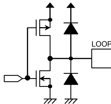
Figure 6 \overline{\text{RST}} Pin (Without Pull-up Resistor)
