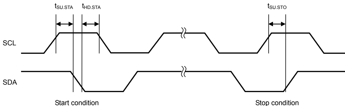
Figure 19 Start / Stop Condition
