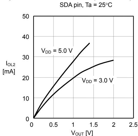
(10) Output current characteristics 2 ( V_{OUT} vs. I_{OL2} )
