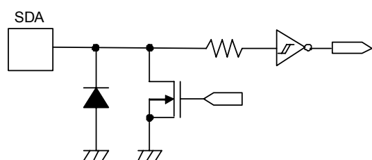
Figure 2 SDA Pin
