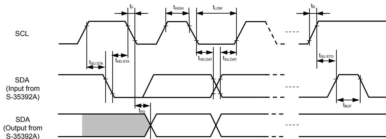
Figure 7 Bus Timing
