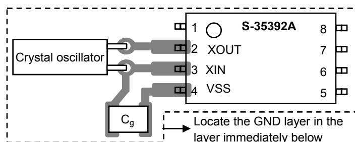
Figure 46 Connection Diagram 2
