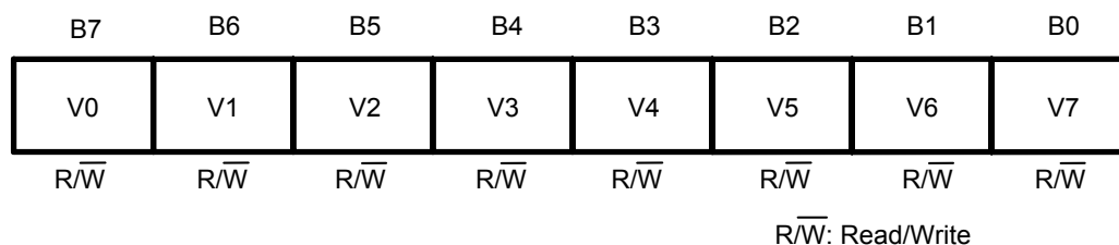
Figure 16 Clock-Correction Register
