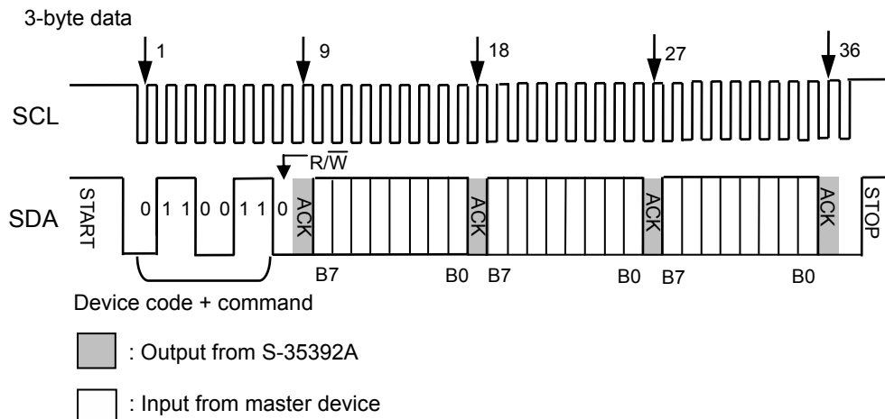
Figure 33 Example of Data Read 2 (3-Byte Data Register)
