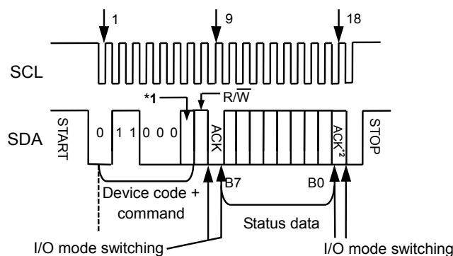
Figure 36 Status Register 1 Access and Status Register 2 Access
