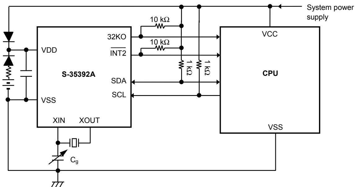
Figure 44 Application Circuit 2
