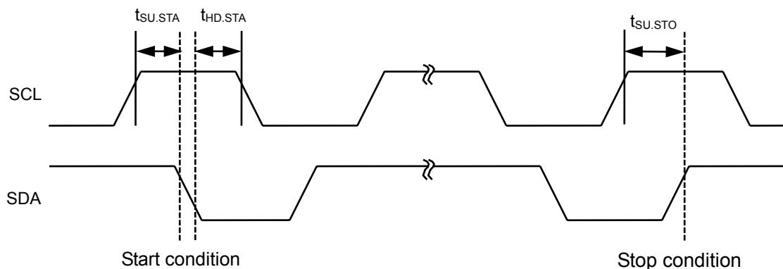
Figure 28 Start/Stop Conditions
