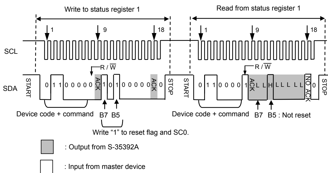
Figure 19 Status Register 1 Data at Initialization
