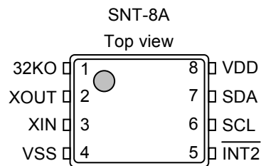
Figure 1 Pin Configuration (S-35392A-I8T1G)
