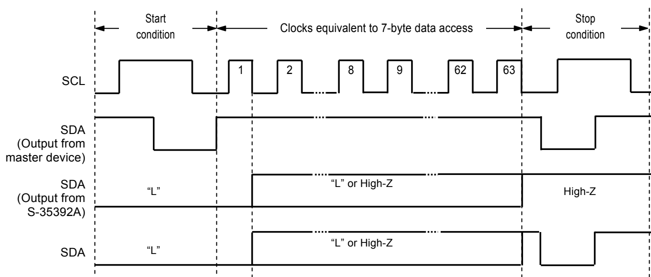
Figure 41 How to Reset
