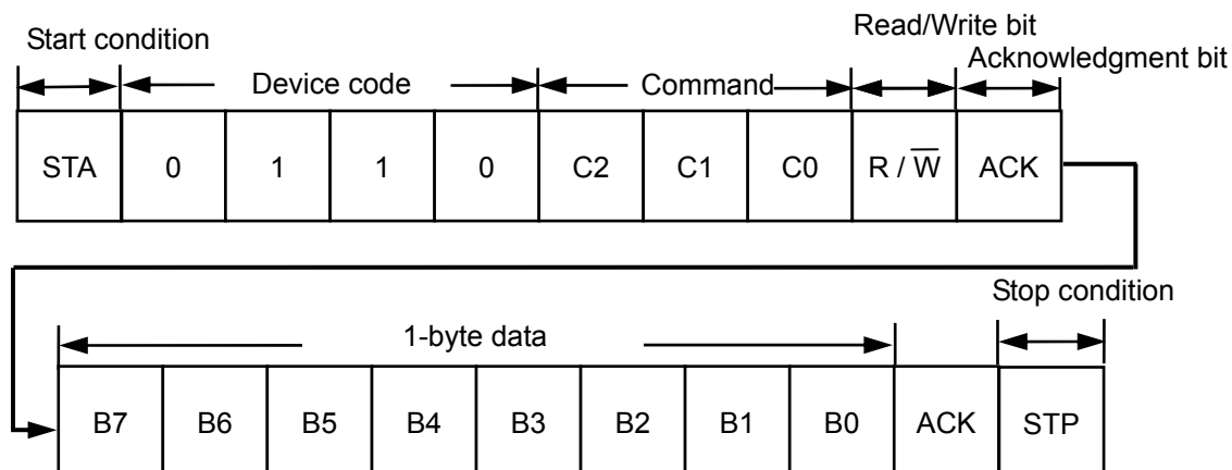
Figure 8 Data Communication
