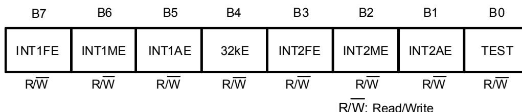
Figure 13 Status Register 2
