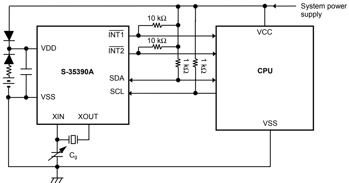
Figure 47 Application Circuit 1
