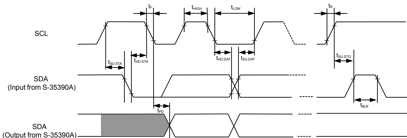
Figure 9 Bus Timing
