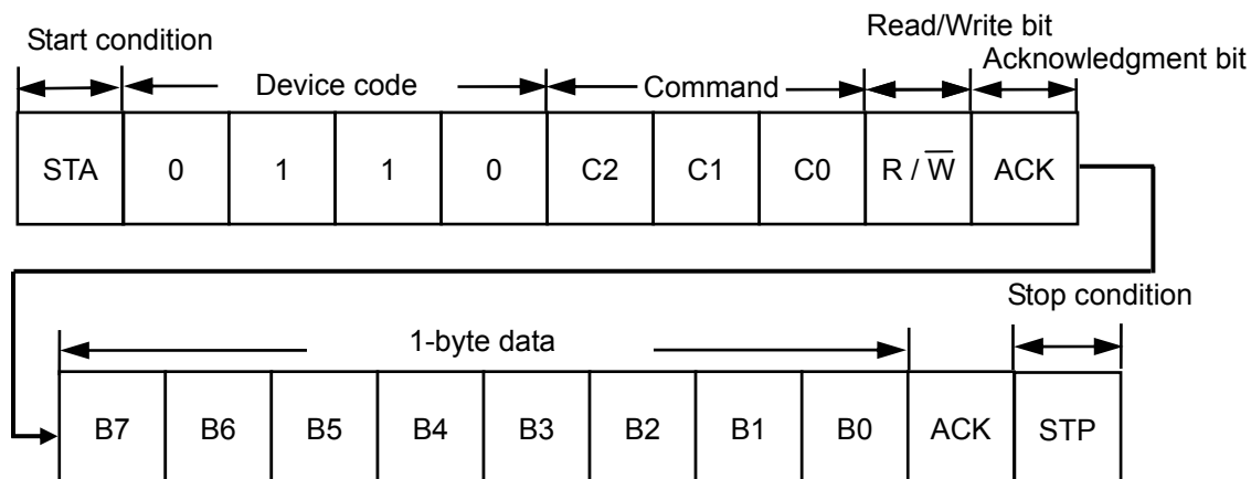
Figure 10 Data Communication
