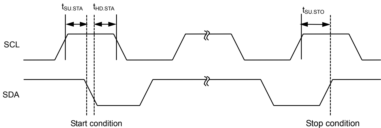
Figure 32 Start/Stop Conditions
