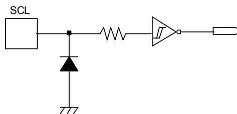
Figure 5 SCL Pin
