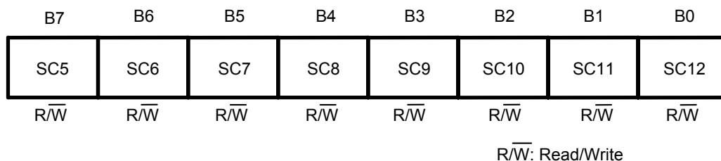
Figure 16 INT Register 1 (Free register)
