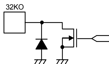
Figure 5 32KO pin
