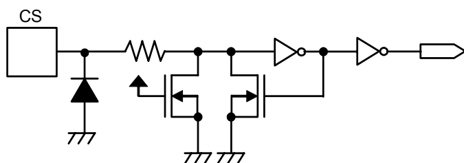
Figure 4 CS pin
