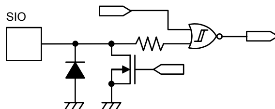
Figure 3 SIO pin
