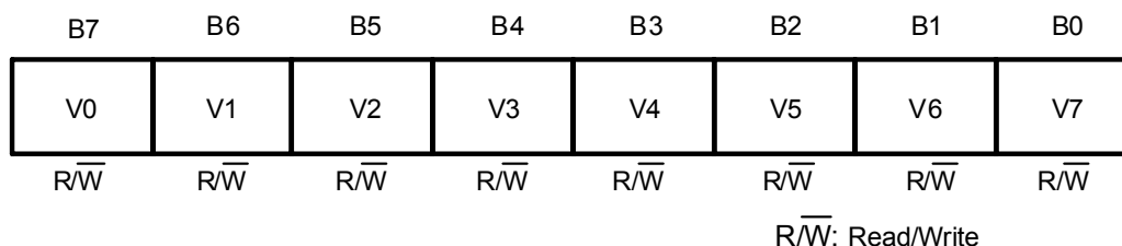
Figure 17 Clock-Correction Register
