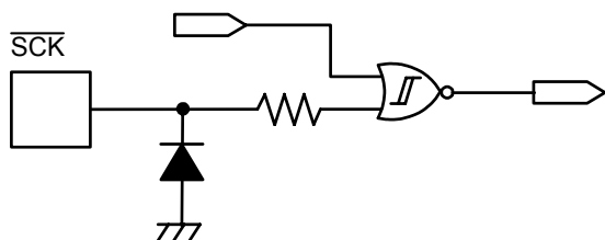
Figure 2 \overline{\text{SCK}} pin
