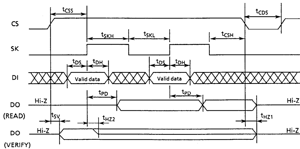
Figure 3 Timing Chart
