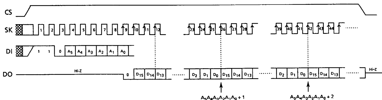
Figure 4 Read Timing (S-29U130A)
