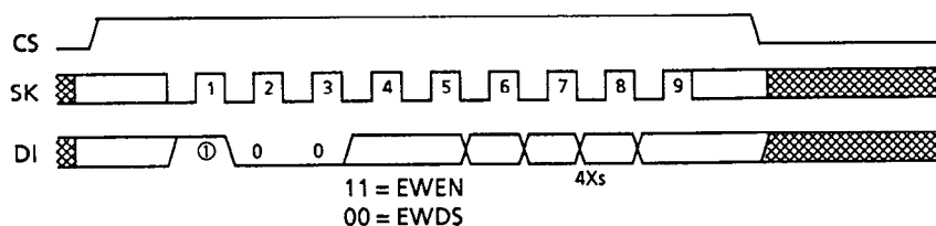
Figure 13 EWEN/EWDS Timing (S-29U130A)
