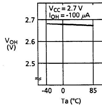
1.13 High level output voltage V_{OH} – Ambient temperature T_a
