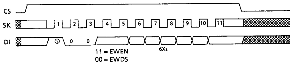
Figure 14 EWEN/EWDS Timing (S-29U220A)
