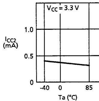
1.5 Current consumption (PROGRAM) I_{CC2} — Ambient temperature T_a
