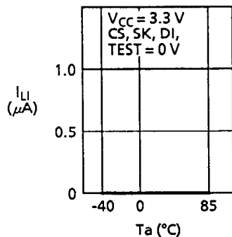
1.9 Input leakage current I_{LI} – Ambient temperature T_a
