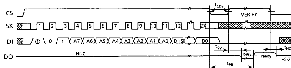
Figure 9 WRITE Timing (S-29U330A)
