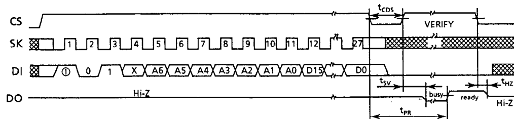
Figure 8 WRITE Timing (S-29U220A)
