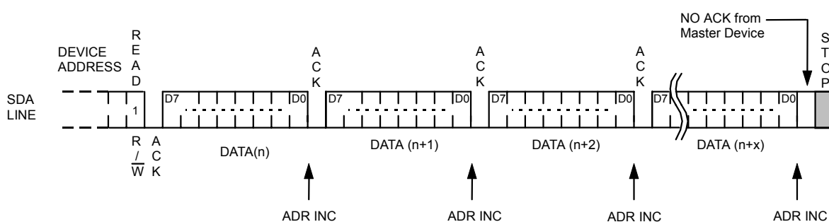
Figure 18 Sequential Read
