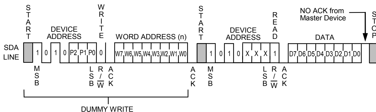
Figure 17 Random Read
