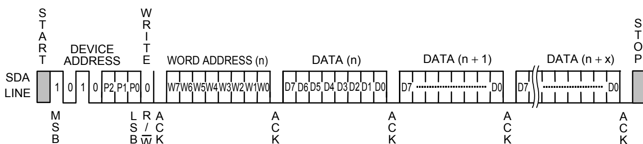
Figure 13 Page Write
