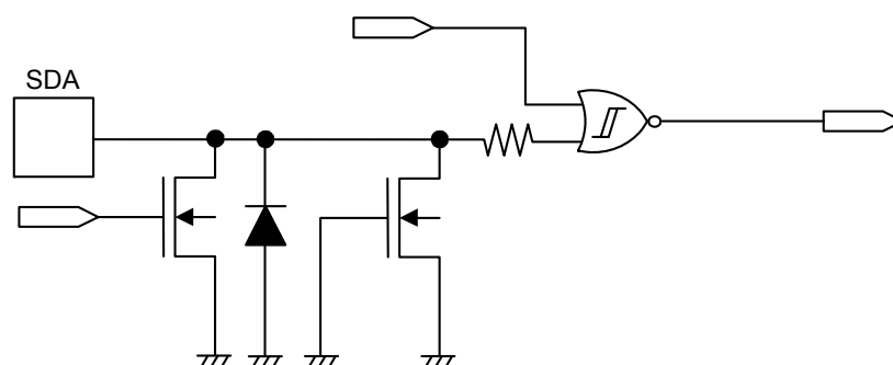
Figure 21 SDA Pin
