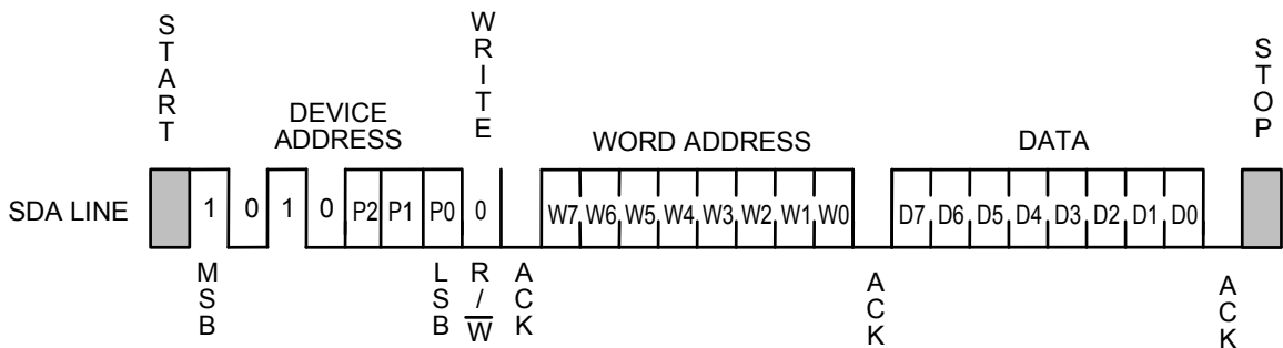
Figure 12 Byte Write
