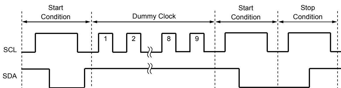
Figure 23 Resetting S-24C08C
