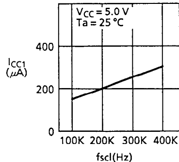
1.7 Current consumption (READ) I_{CC1} — Clock frequency f_{scl}
