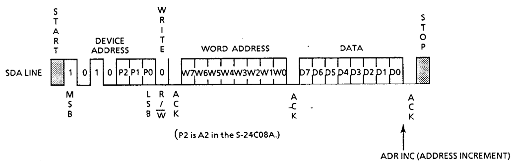
Figure 10 Byte Write
