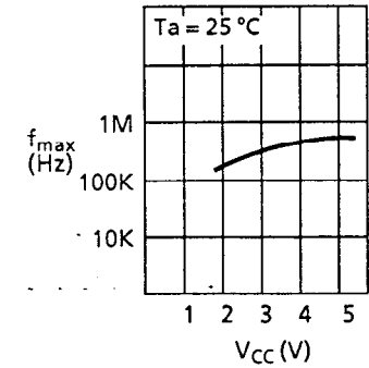
2.1 Maximum operating frequency f_{max} — Power supply voltage V_{CC}
