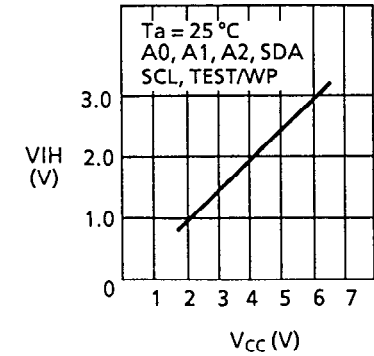
1.23 High input inversion voltage V_{IH} — Power supply voltage V_{CC}
