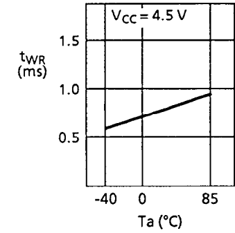
2.3 Write time t_{WR} — Ambient temperature T_a
