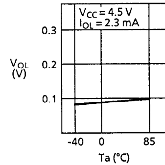
1.19 Low level output voltage V_{OL} — Ambient temperature T_a
