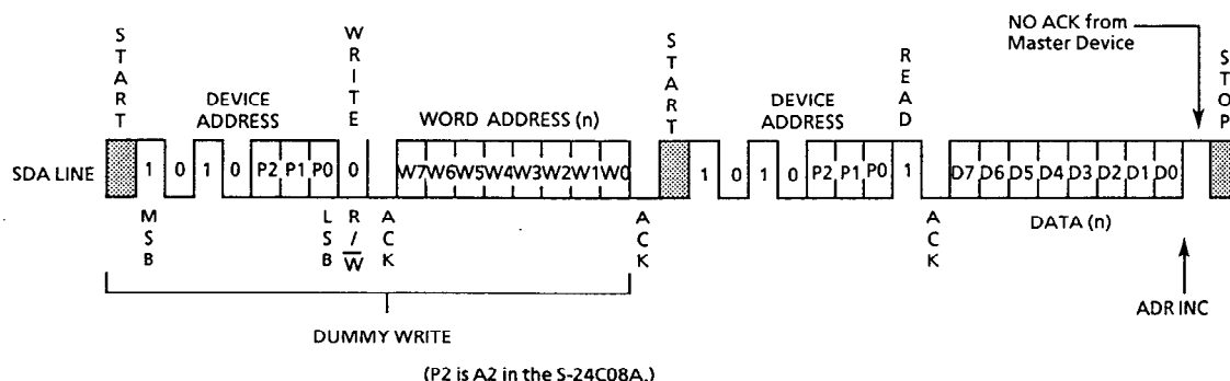
Figure 13 Random Read
