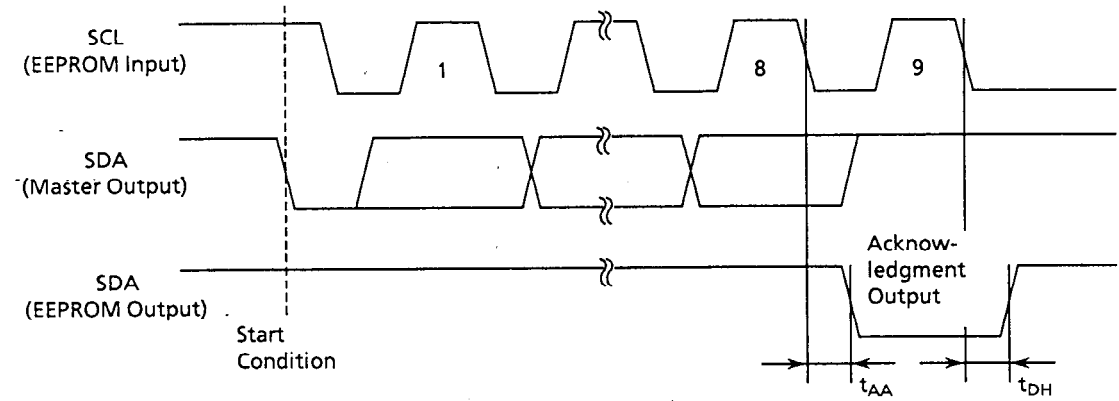
Figure 8 Acknowledgment Output Timing
