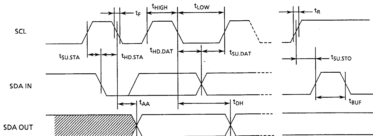
Figure 4 Bus Timing
