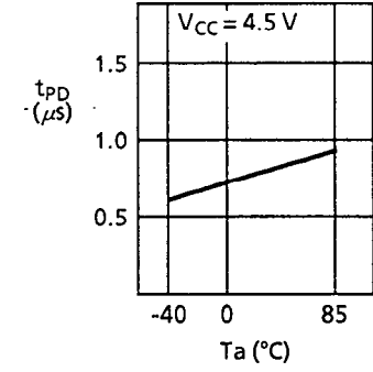
2.5 SDA output delay time t_{PD} — Ambient temperature T_a
