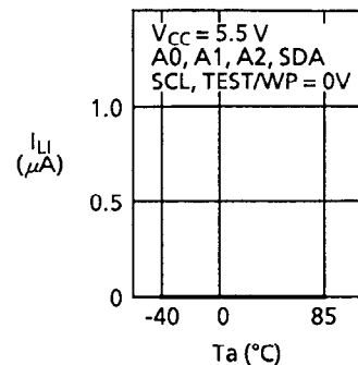
1.15 Input leakage current I_{LI} — Ambient temperature T_a
