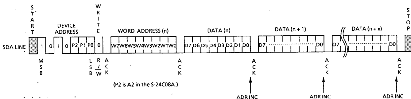
Figure 11 Page Write
