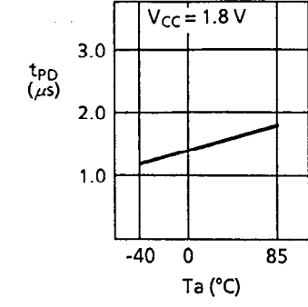
2.7 SDA output delay time t_{PD} — Ambient temperature T_a
