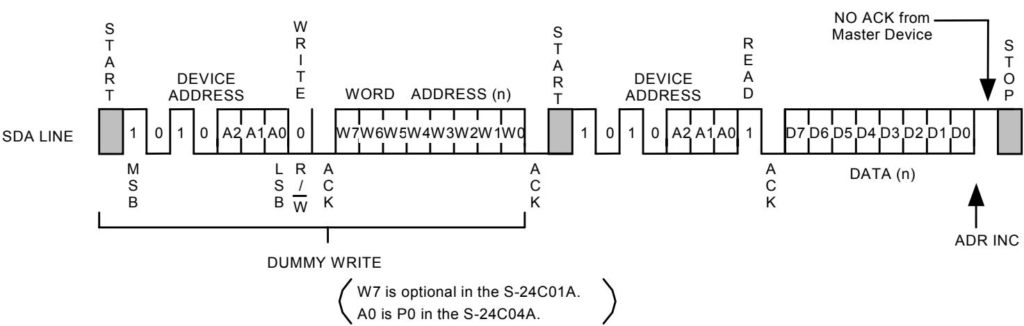
Figure 13 Random Read
