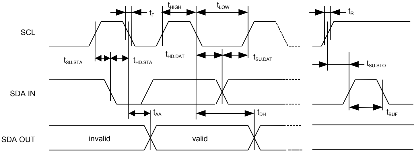
Figure 4 Bus Timing
