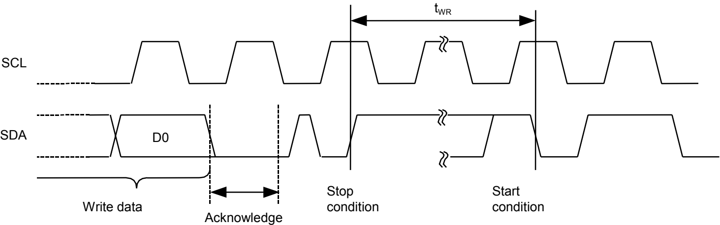
Figure 5 Write Cycle
