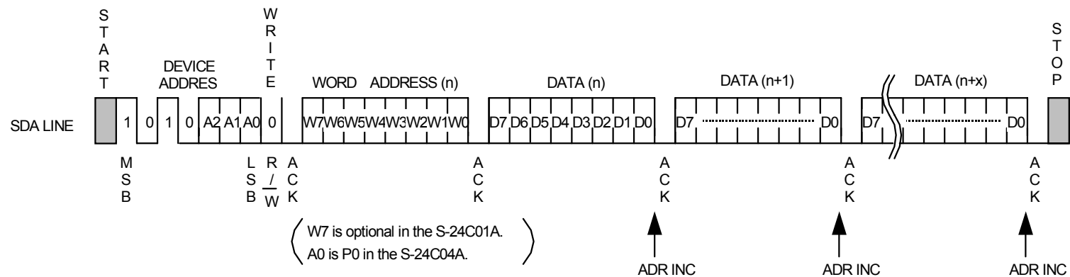
Figure 11 Page Write
