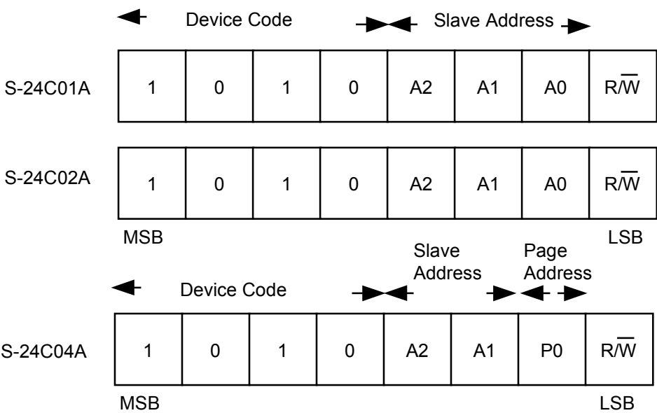
Figure 9 Device Address
