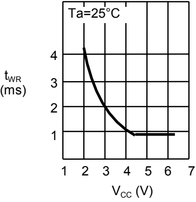
2.2 Write time t_{WR} – Power supply voltage VCC
