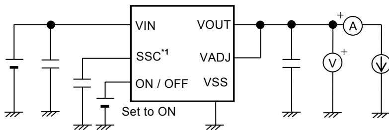
Figure 16 Test Circuit 8
