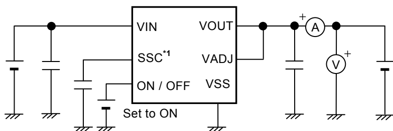
Figure 18 Test Circuit 10
