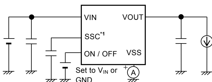
Figure 10 Test Circuit 2
