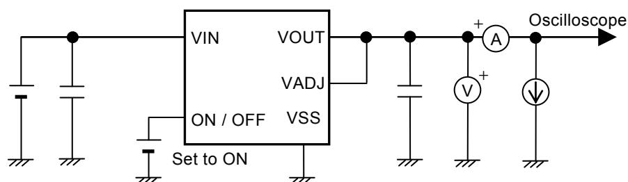
Figure 22 Test Circuit 14
