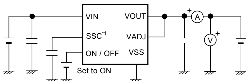
Figure 18 Test Circuit 10
