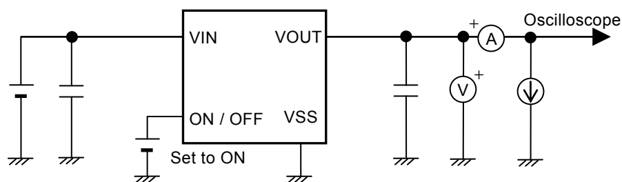
Figure 15 Test Circuit 7
