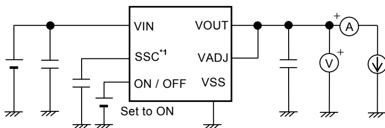
Figure 16 Test Circuit 8
