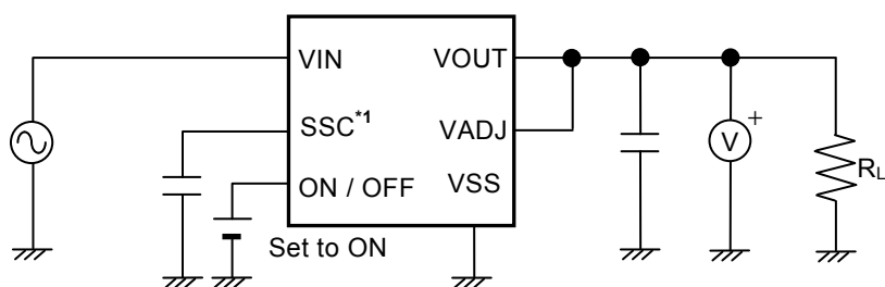
Figure 20 Test Circuit 12
