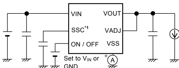
Figure 17 Test Circuit 9
