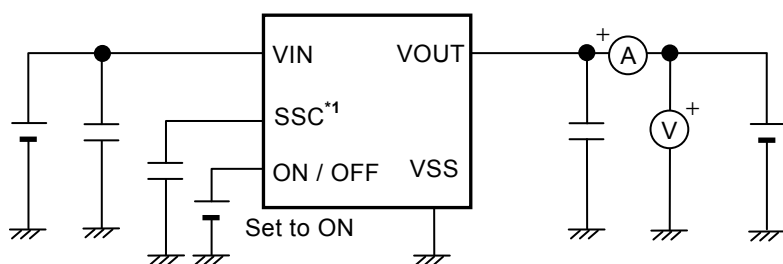
Figure 11 Test Circuit 3
