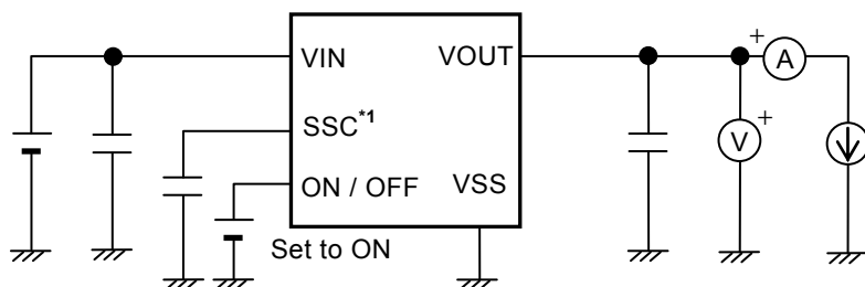
Figure 9 Test Circuit 1
