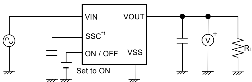
Figure 13 Test Circuit 5
